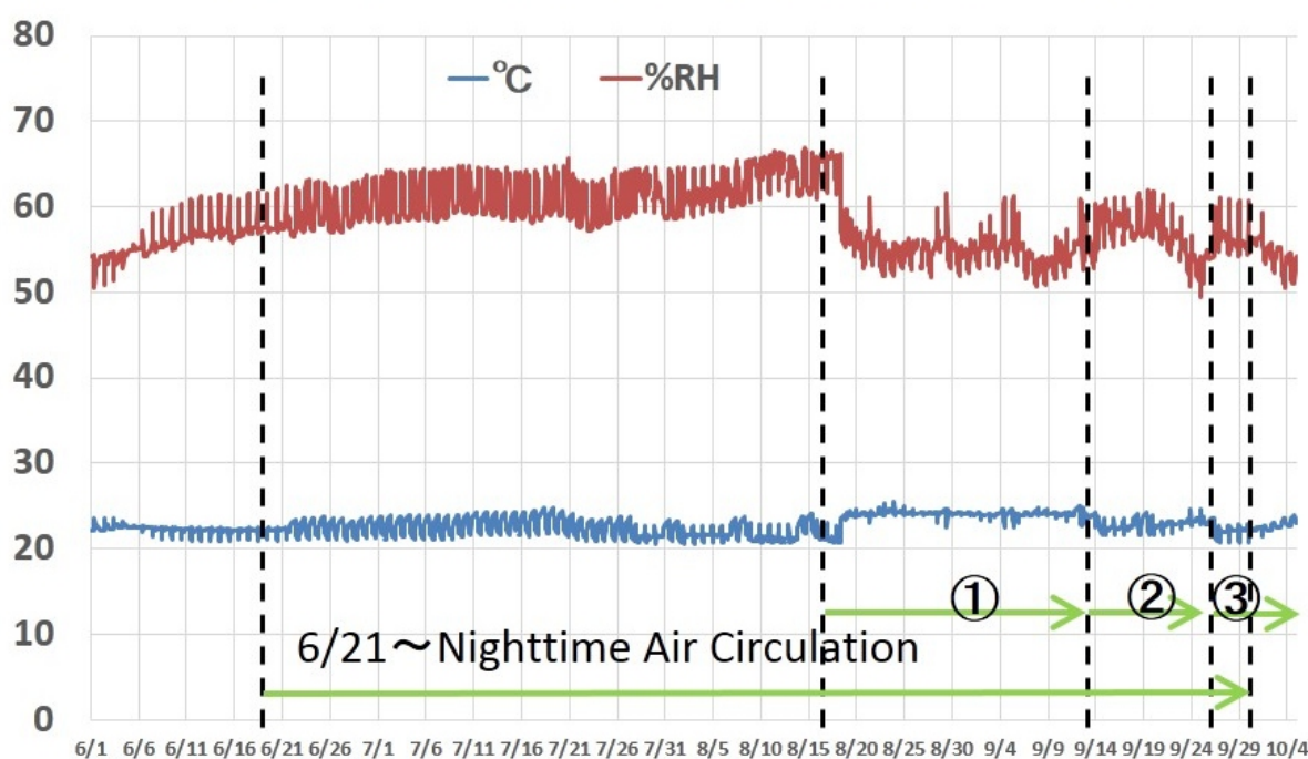
Temperature and Humidity in Layer 14, Area 3, 6/1 ~ 10/4, 2011
