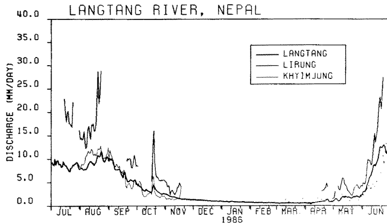
Fig. 4. Yearly variations in the daily discharge rate of the Langtang Khola Watershed, the Lirung Khola Watershed and the Khyimjung Glacier Watershed
