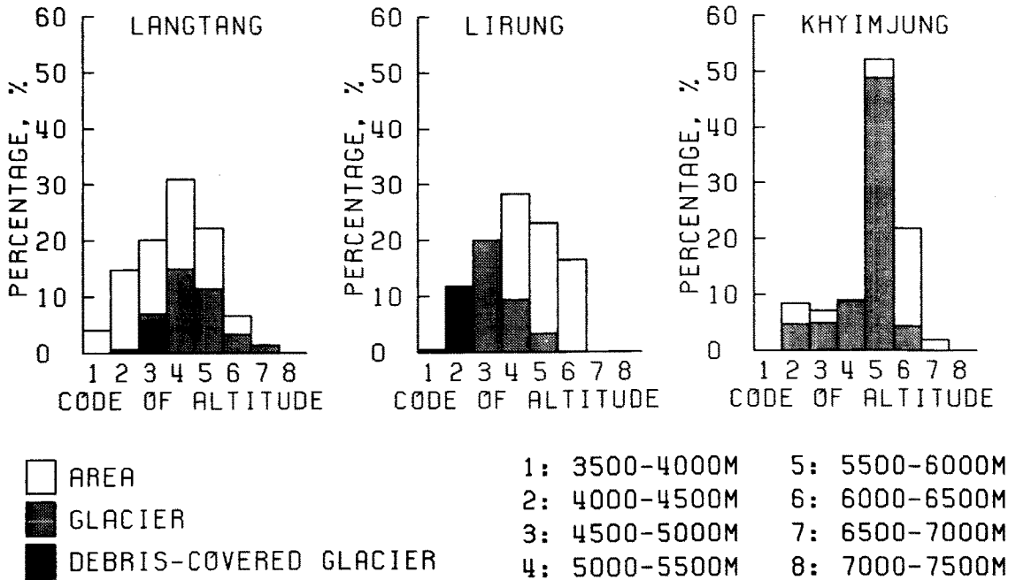
Fig. 2. The distributions of the drainage basins and the glaciers included in the altitude at 500 m intervals in each watershed
