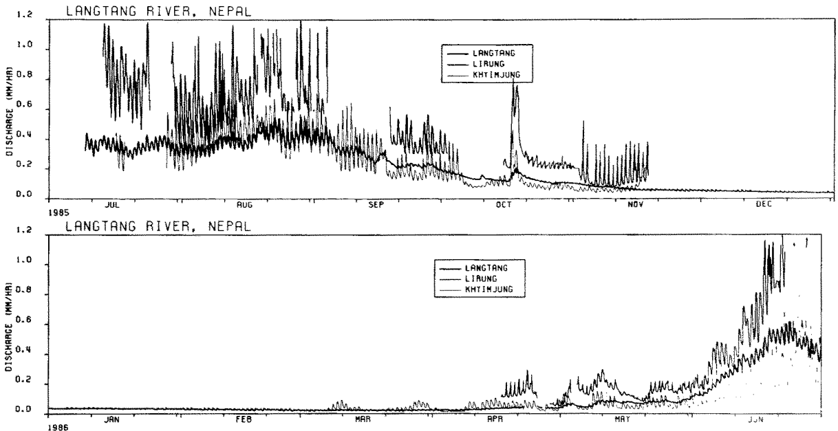
Fig. 5. Yearly variations in the hourly discharge rate of three watersheds
