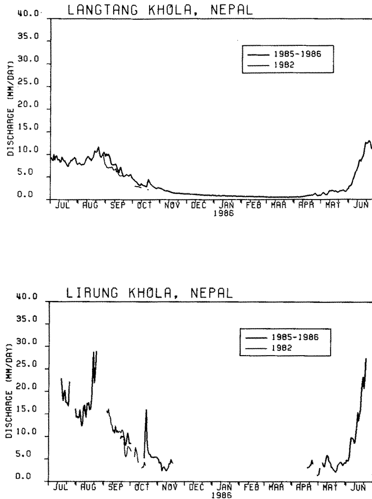
Fig. 7. Comparison of both daily discharge rates observed in 1985-86 and 1982 (Yamada et al. , 1984), of the Langtang K.W. and the Lirung K.W.
