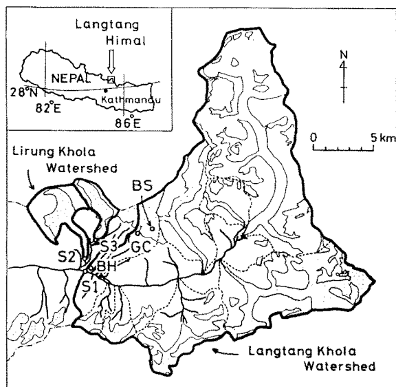
Fig. 1. A topographical map of the Langtang Valley. The thick solid lines indicate the boundaries of the Langtang Khola Watershed (observation site : S1), The Lirung Khola Watershed (observation site : S2) and The Khyimjung Glacier Watershed (observation site : S3). BH : Base House for meteorological observations.
