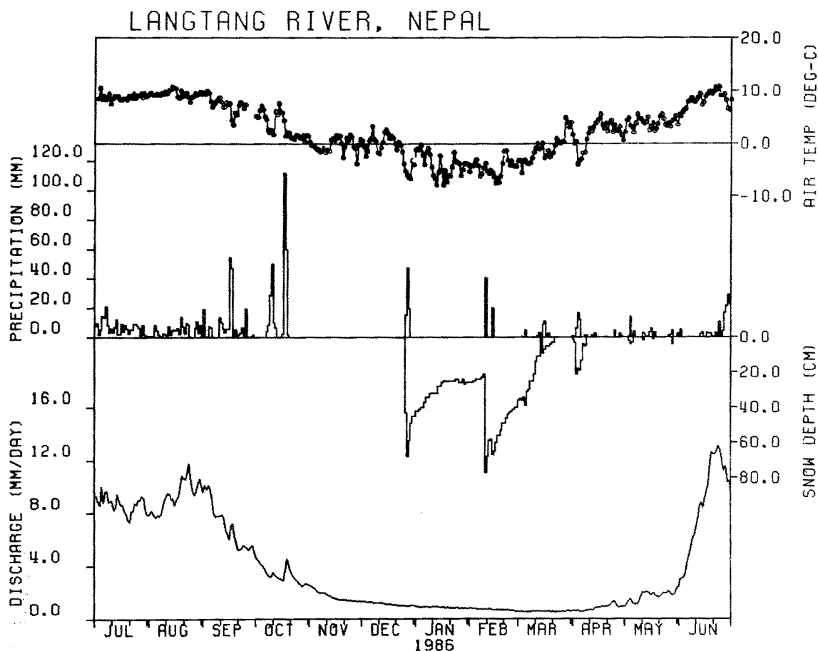
Fig. 3. Yearly variations in the daily precipitation, the daily mean air temperature and the snow depth at BH in Kyangchen, and the discharge rate at S1, the site of the Langtang Khola W. (basin area : 333km 2 )
