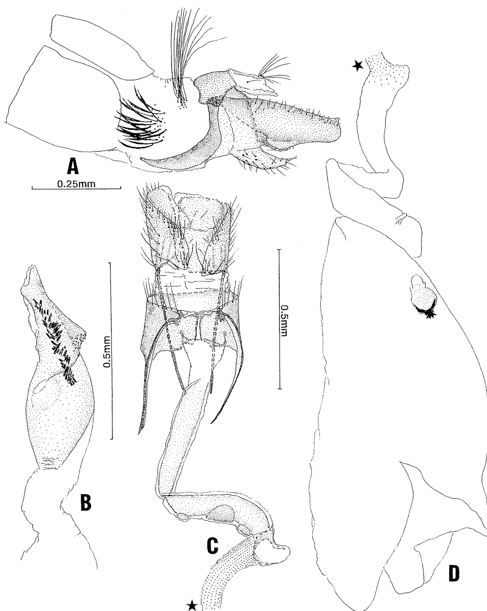
Fig. 1. Monochroa cleodora (MEYRICK). A: Male genitalia in lateral view, aedeagus omitted [Gel-93025, Mt. Ishizuchi, Ehime Pref., 20/vii/1961, M. OKADA leg.]. B: Aedeagus [ditto]. C: Female genitalia in ventral view, apical part of bursa copulatrix omitted [Gel-93026, ditto]. D: Apical part of bursa copulatrix [ditto].
