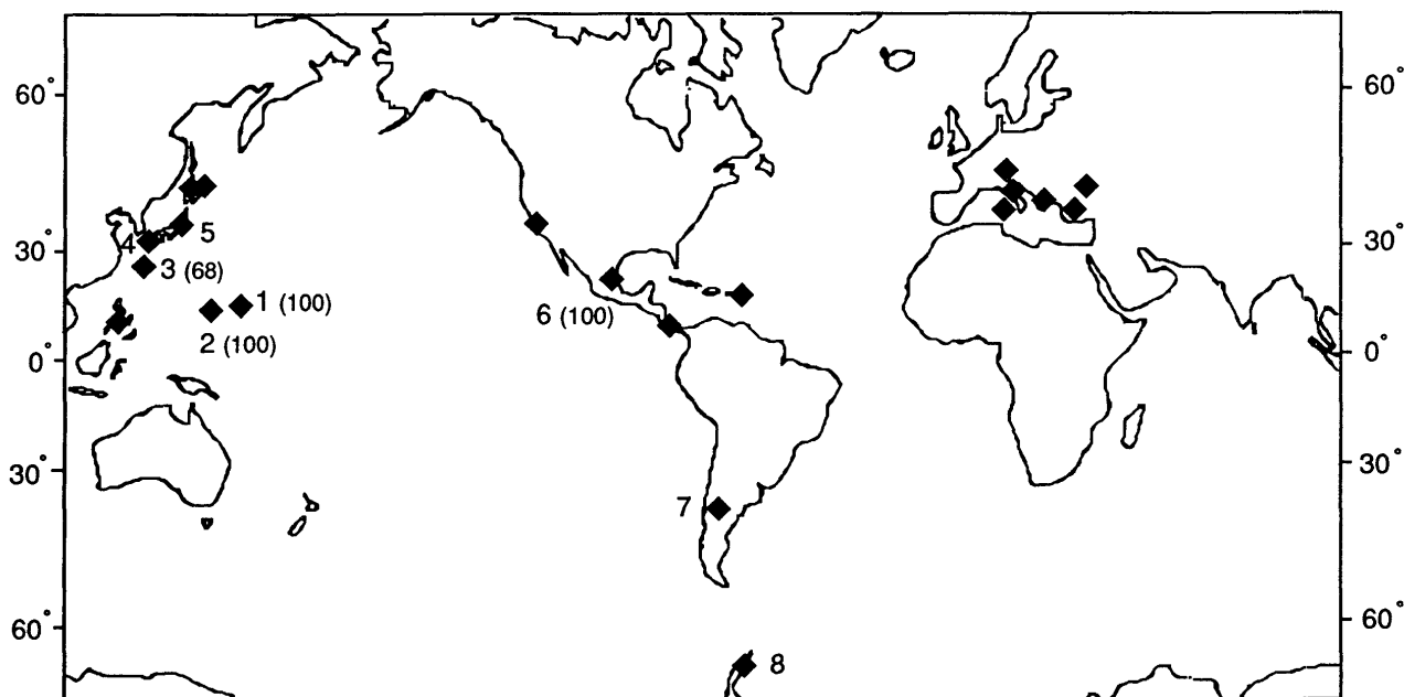
Fig. 6. Occurrences of the Vallupus group in the world. Localities with number are referred in the text. Numbers in parentheses indicate VEN in KR1 ( Pseudodictyomitra carpatica Zone). 1: ODP Site 801, 2: Mariana Trench, 3: Ie Island, Ryukyu Arc, 4: Ebirase Formation, western Kyushu, 5: Yamizo Mountains, 6: Taman Formation, 7: Neuquen Basin, 8: Antarctic Peninsula.
