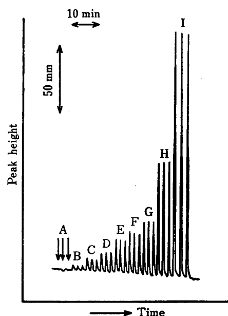
Fig. 4 Flow signals for ammoniacal nitrogen
