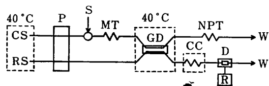
Fig. 1 Schematic diagram of flow system
