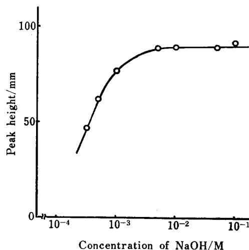
Fig. 3 Effect of sodium hydroxide in carrier solution on the peak height
