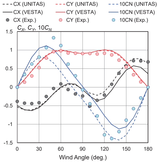
Fig. 17 Validation for vehicle carrier ( L_{OA} = 199 m)
