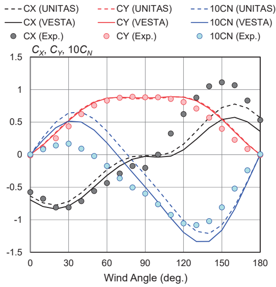
Fig. 15 Validation for container ship ( L_{OA} = 312 m)
