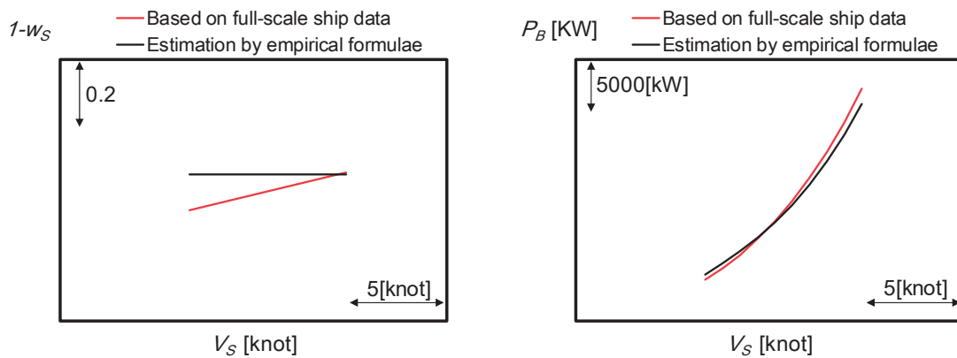
Fig. 19 Comparison between ‘Based on full-scale ship data’ and ‘Estimation by empirical formulae’ for a container ship ( L_{PP} = 300 m)
