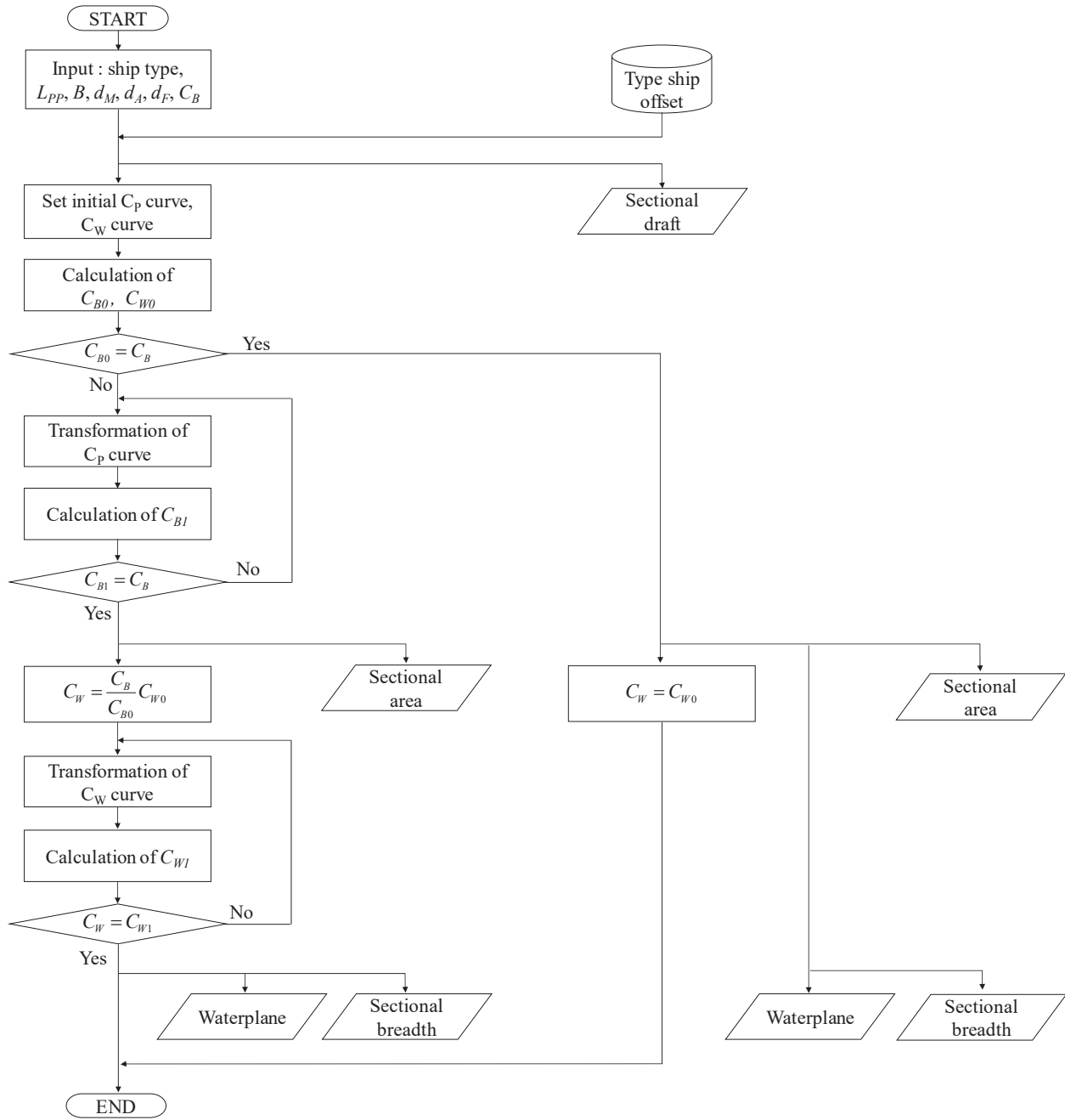
Fig. 3 Flowchart of estimating sectional parameters from principal particulars
