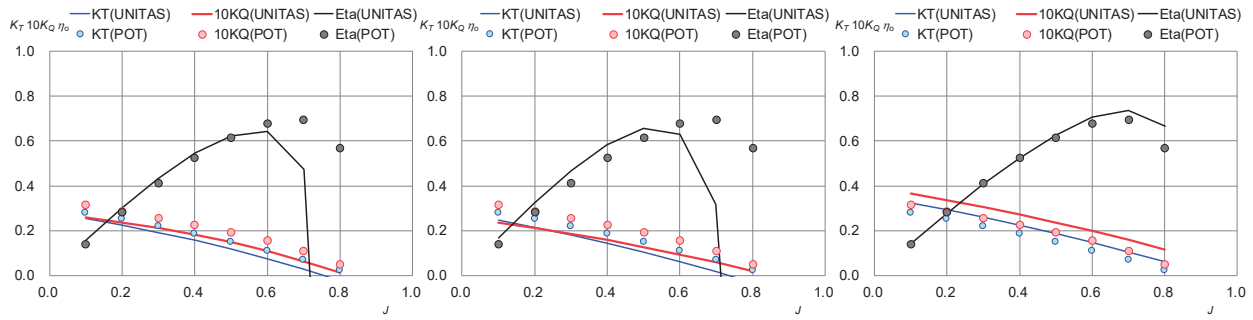
Fig. 10 Validation for POC of 33CT
