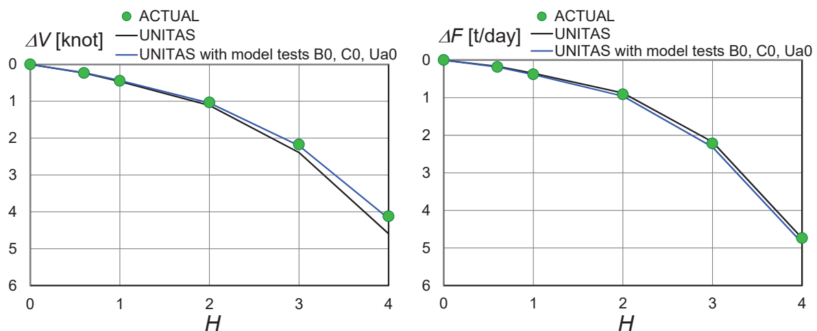
Fig. 25 Results of ship performance simulation. (left: decrease in ship speed ( \Delta V ), right: increase in FOC per day ( \Delta F ))
