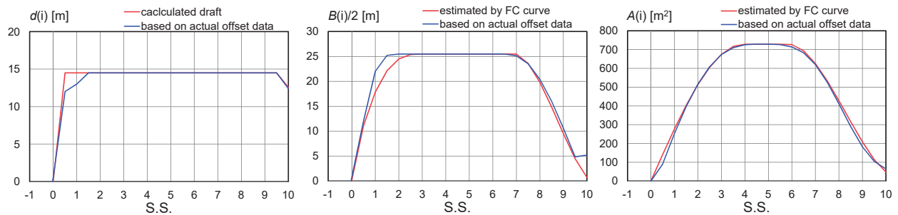
Fig. 6 Validation for sectional parameters of DTC (left: draft, center: half breadth, right: sectional area)
