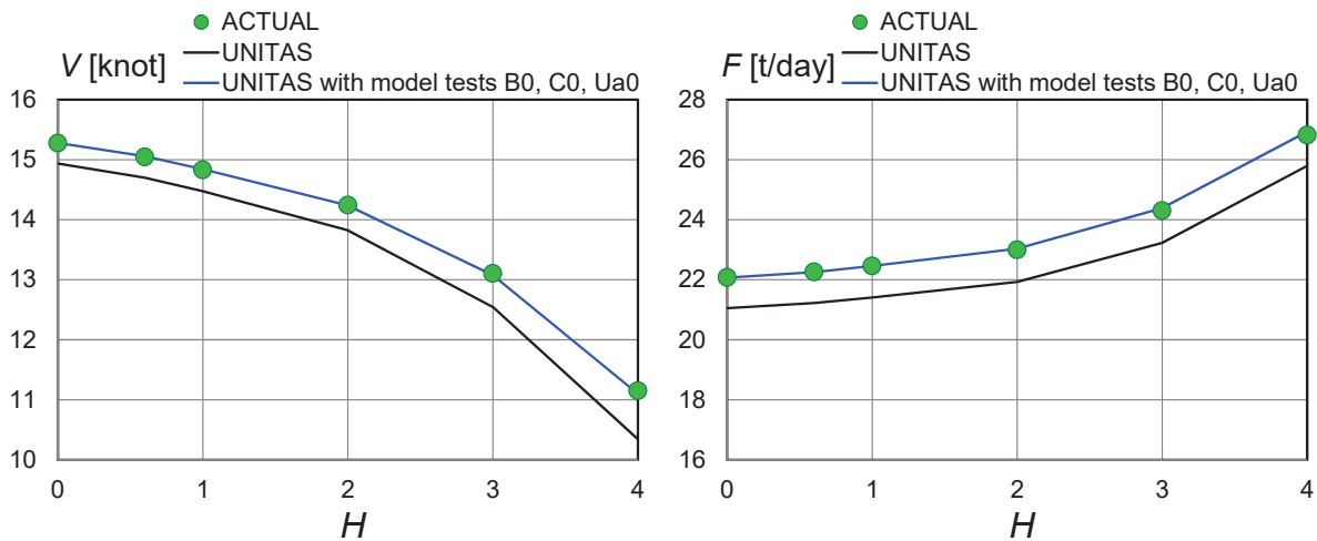
Fig. 24 Results of ship performance simulation (left: ship speed ( V ), right: FOC per day ( F ))
