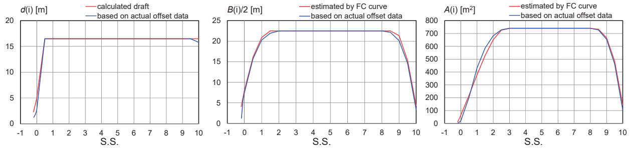
Fig. 5 Validation for sectional parameters of JBC (left: draft, center: half breadth, right: sectional area)
