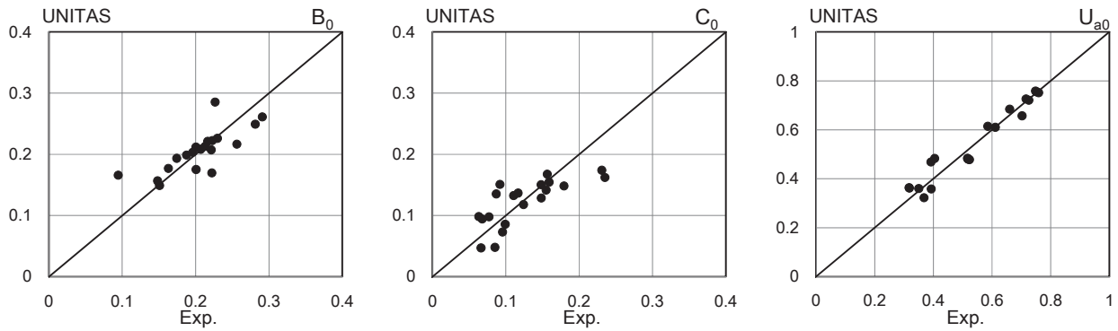
Fig. 21 Comparison of coefficients in load variation method
