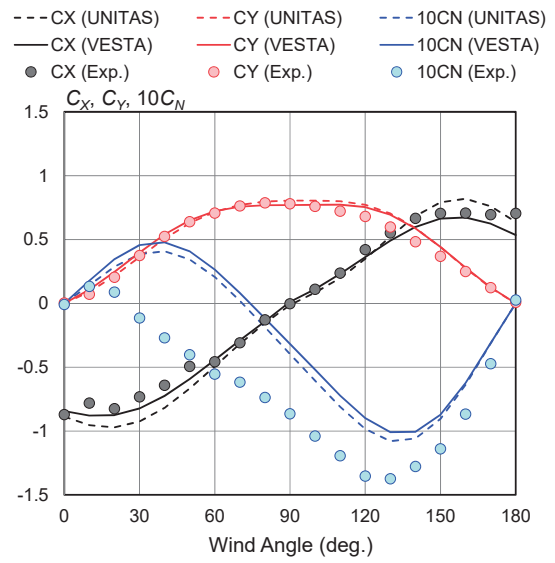
Fig. 16 Validation for JBC ( L_{OA} = 291.2 m)
