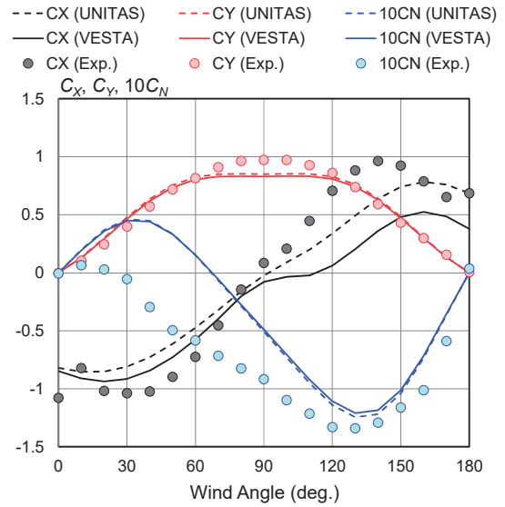
Fig. 18 Validation for 33CT ( L_{OA} = 178 m)
