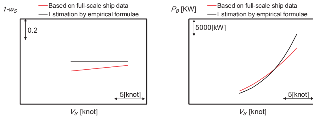
Fig. 20 Comparison between ‘Based on full-scale ship data’ and ‘Estimation by empirical formulae’ for vehicle carrier ( L_{PP} = 192 m)
