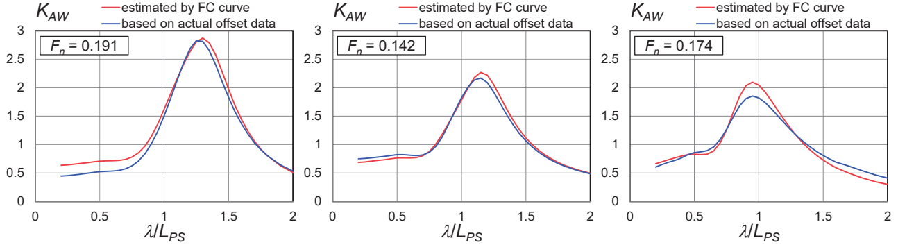
Fig. 7 Added resistance in regular heading waves (left: 33CT, center: JBC, right: DTC)
