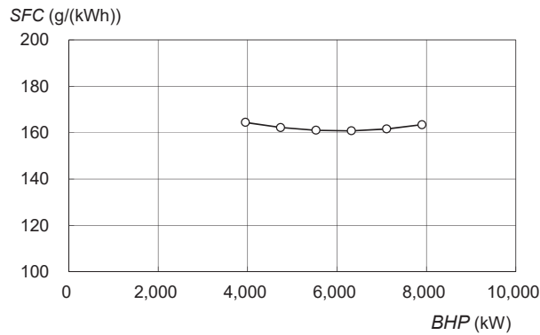
Fig. 23 Specific fuel oil consumption (SFC) of engine
