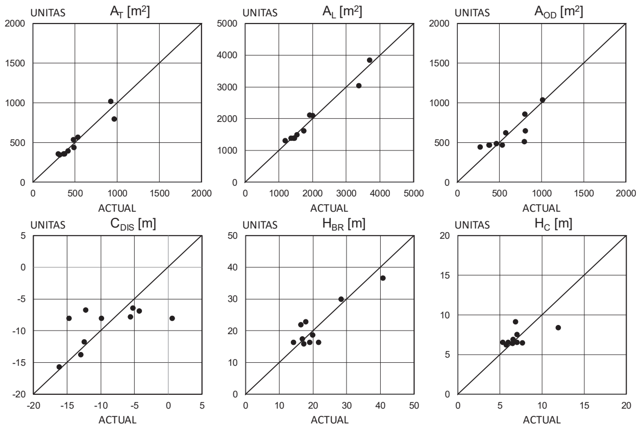
Fig.14 Comparison of superstructure parameters (bulk carriers in full condition)
