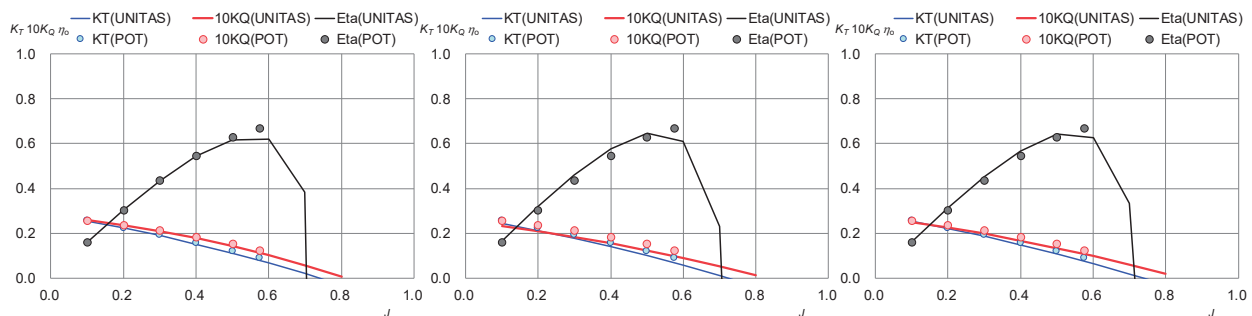
Fig. 9 Validation for POC of 499GT cargo ship
