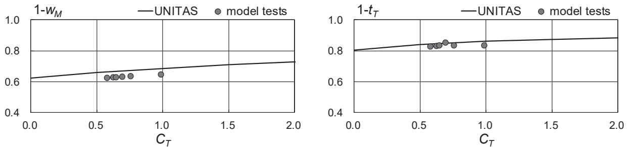
Fig. 22 Comparison of 1-w_M and 1-t_T for 33CT between UNITAS and model tests
