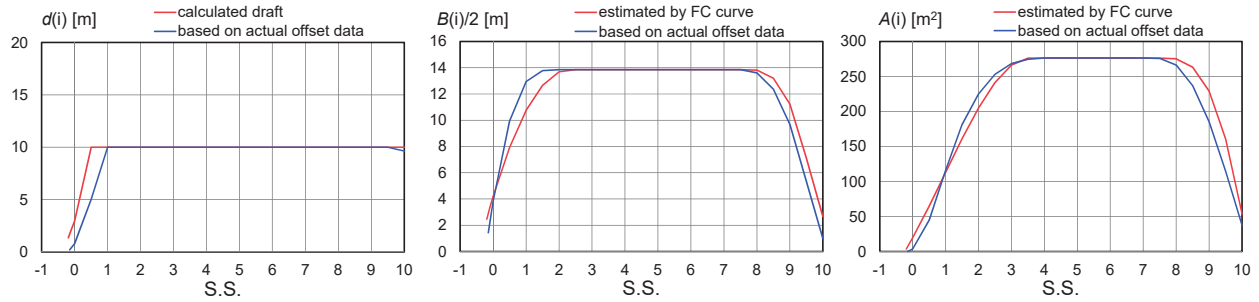
Fig. 4 Validation for sectional parameters of 33CT (left: draft, center: half breadth, right: sectional area)
