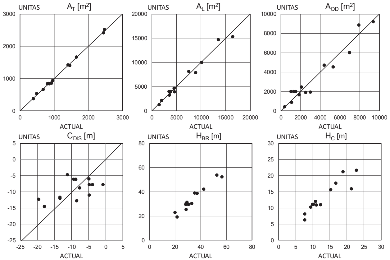
Fig.13 Comparison of superstructure parameters (container ships)
