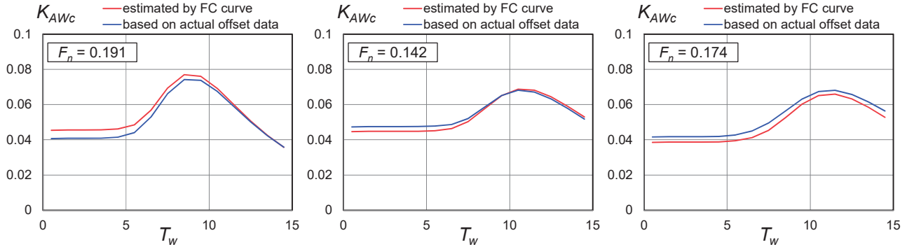
Fig. 8 Added resistance in short crested irregular waves where primary direction is heading (left: 33CT, center: JBC, right: DTC)
