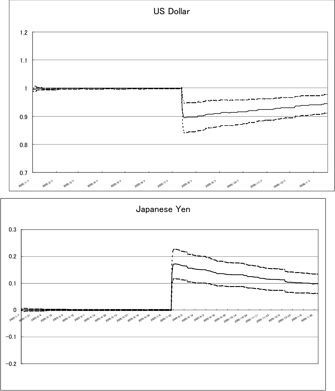
Figure 3: Results of Estimation by using Kalman Filter Method (model without Korean Won)
