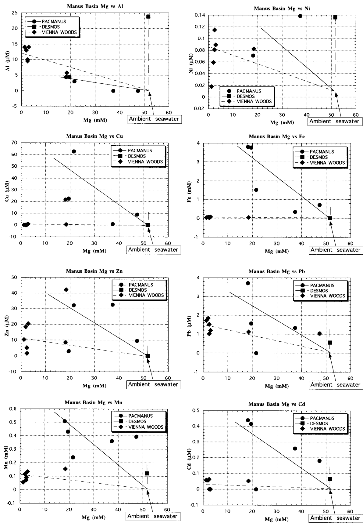
図3 マナス海盆の各熱水域から採取した熱水試料のMgに対する微量元素(Al, Ni, Fe, Cu, Zn, Pb, Mn, Cd)のプロット Fig. 3 Relationships between Mg and Al, Ni, Fe, Cu, Zn, Pb, Mn and Cd for hydrothermal fluids collected at PACMANUS, DESMOS and VIENNA WOODS hydrothermal sites during the cruise.
