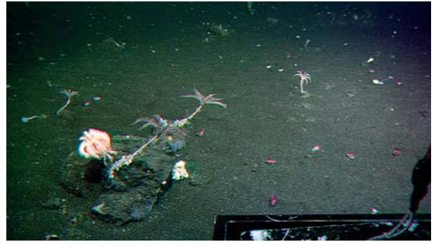
図8 海形海山南西部斜面に数メートルおきに点在する転石上の生物群集と多数のダンゴイカ類。 Fig. 8 Biological communities on rocks scattered one every few meters, and many sepiolid cephalopods, were observed on the southwestern slope of the Kaikata Seamount.
