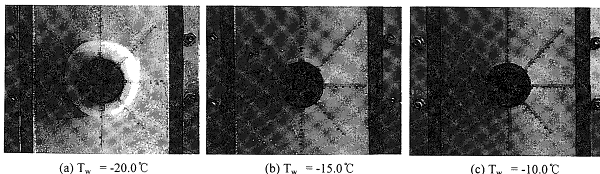
Fig.10 Effect of cooled-tube temperature on freezing behavior ; Q_{\text{air}} = 10\text{L/min} , U_i = 0.02\text{m/s}
