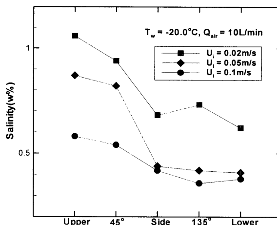
Fig.6 Salt concentration of frozen layer except the initial freezing
