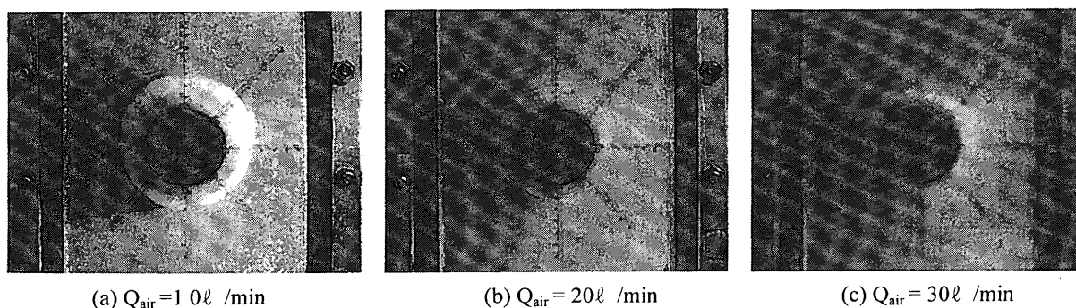
Fig.8 Effect of air-bubble flow rate on freezing behavior ; U_i = 0.02 \text{ m/s} , T_w = -20^\circ \text{C}
