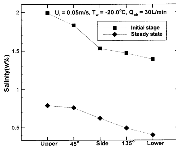
Fig.3 Salinity distribution of frozen layer
