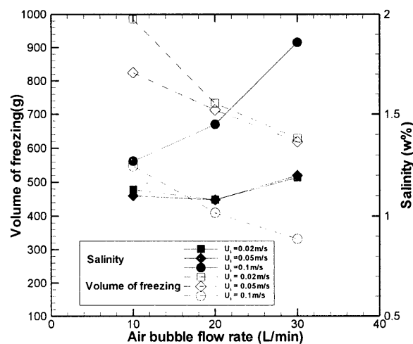
Fig.9 Effect of air-bubble flow rate on salt concentration of frozen layer
