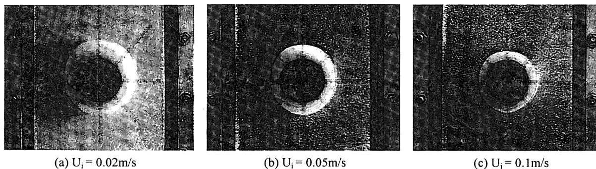
Fig.5 Effect of fluid velocity on freezing behavior ; Q_{air} = 10\text{L/min} , T_w = -20^\circ\text{C}
