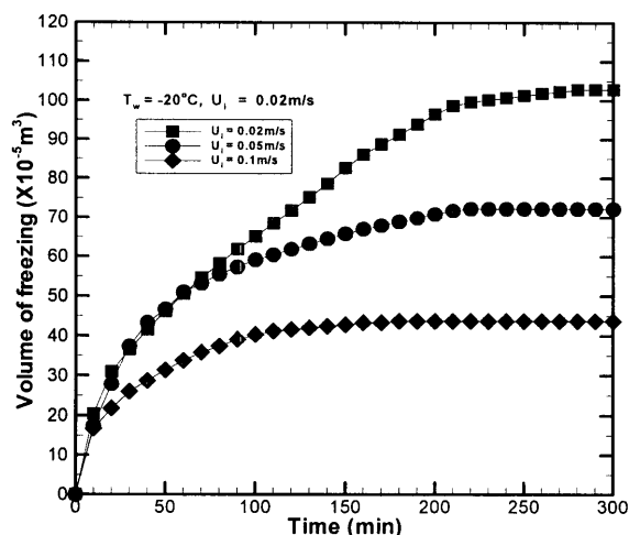
Fig.4 Effect of fluid velocity on freezing rate
