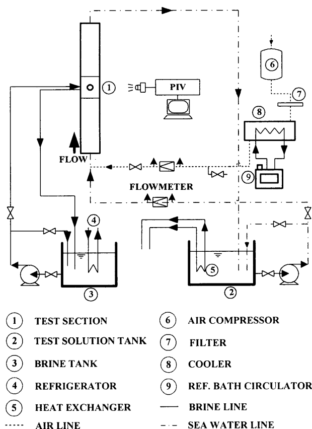
Fig.1 Schematic of experimental apparatus
