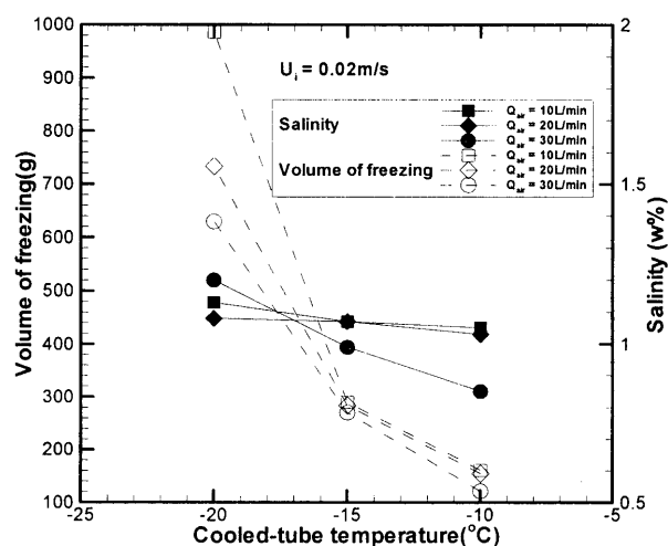
Fig.11 Effect of cooled-tube temperature on salt concentration of frozen layer
