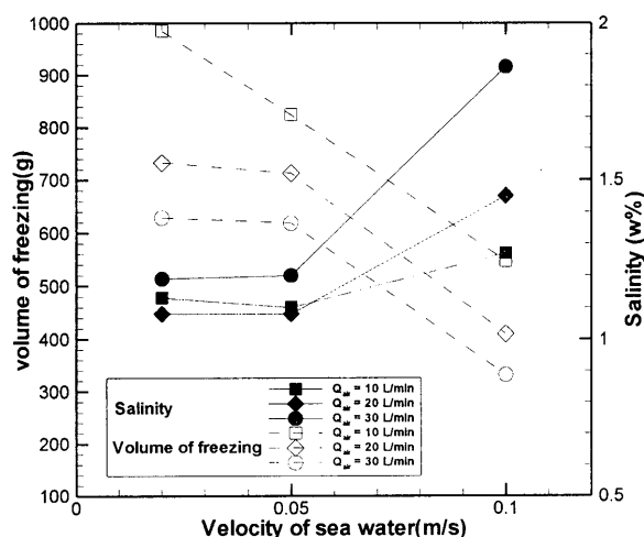
Fig.7 Salt concentration of steady-state frozen layer
