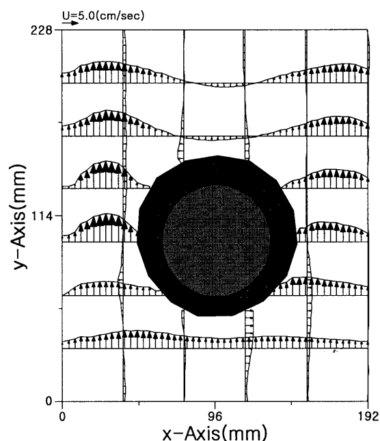
Fig.2 Time-mean velocity profile
