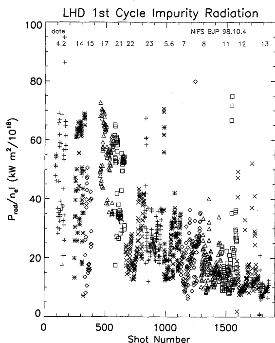
Fig. 4 Radiation loss per density measured with bolometer in the first campaign of LHD.
