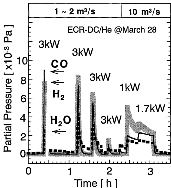
Fig. 1 Gas desorption under the first ECR discharge cleaning in LHD.
