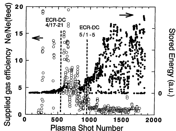
Fig. 5 Improvement of gas efficiency and plasma stored energy with wall conditioning in LHD, where the gas efficiency defines the ratio of averaged plasma density to electron density supplied by gas-puffing.
