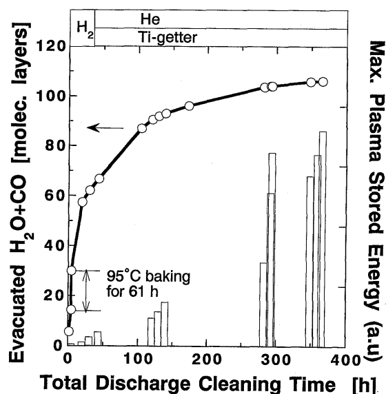
Fig. 3 Results of ECR-DC in the first campaign of LHD.
