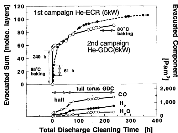
Fig. 8 Gas evacuation under GDC in the second campaign in comparison to ECR in the first campaign of LHD.
