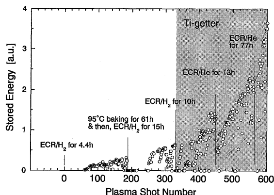
Fig. 6 The effect of Ti-gettering on the plasma stored energy in the first campaign of LHD.
