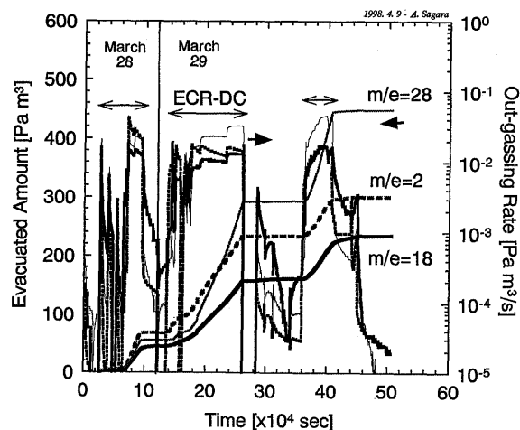
Fig. 2 Outgassing and evacuation under various ECR-DC tests before the LHD first shot.
