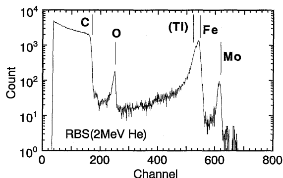
Fig. 7 RBS spectrum of the graphite sample exposed to the divertor plasma in the first campaign of LHD.
