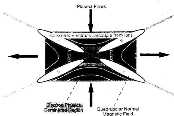
Fig. 4 The Hall current loop in the proximity of the reconnection region. Within the ion-electron decoupling region, ions are stagnant while electrons are flowing-in vertically and flowing-out horizontally. These facts result in the current loop within the plane and the magnetic field component out of the plane. This Hall effect makes the structure of the out-flow region (the out-flow velocity and the width) to be related to the property of the in-flow, and thus resolving the “choking” problem that makes the Sweet-Parker model to result in slow reconnection [15].
