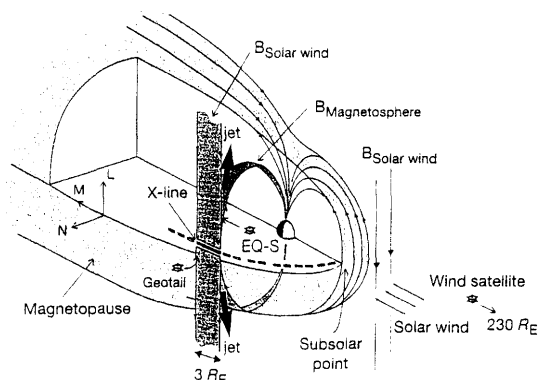
Fig. 2 Observations of large scale quasi-steady dayside reconnection under steady southward interplanetary field. Reconnection is identified to be operative close to the dawn terminator by two spacecrafts which are 3 Earth radii azimuthally apart from each other. Well documented high occurrence probability of reconnection at the subsolar region for southward interplanetary field suggests that the length of the reconnection line is not only comparable to 3 Earth radii but should be extended all the way to the noon. From the symmetry argument, it must have further extended to the dusk terminator [2].
