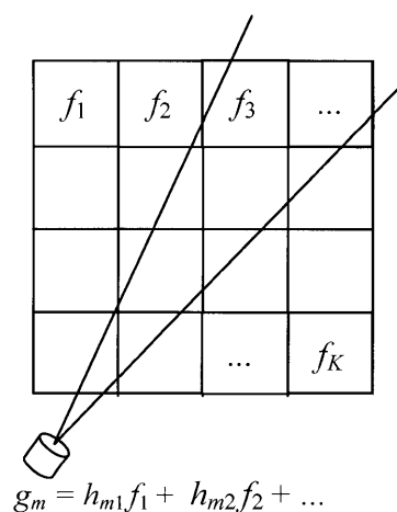
Fig. 3 Pixellation of plasma region and the field of view of a detector for 2D computerized tomography.
