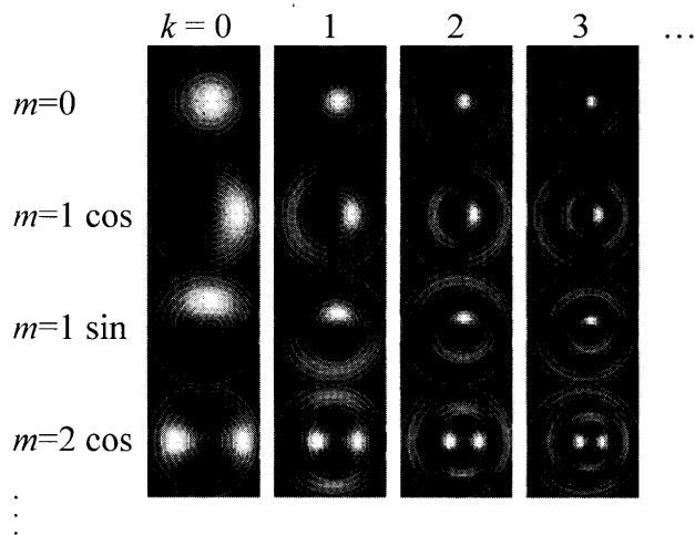
Fig. 4 Fourier-Bessel bases J_m(\lambda_m^{k+1} r) \exp(im\theta) with overlapping display of the magnetic surfaces of TEXTOR tokamak.
