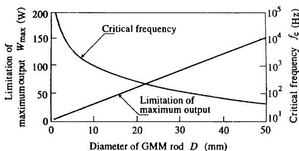
Fig. 3 W_{\max} - D and f_c - D characteristics of GMM (prestress 14 MPa, dimensional ratio 6).
