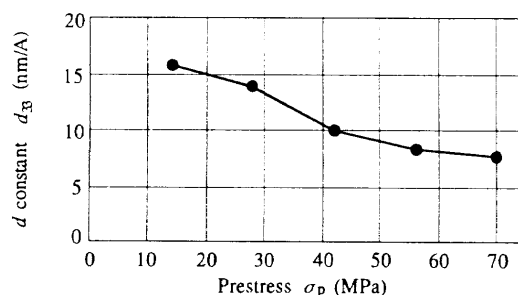
Fig. 2 d_{33} - \sigma_p characteristics of GMM.
