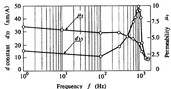
Fig. 5 Frequency characteristics of d_{33} and \mu_r (prestress 13.5 MPa, exciting current 600 mA).
