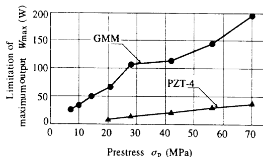
Fig. 1 W_{\max} - \sigma_p characteristics ( f_0=200 Hz, material size \phi 20 \times 120 mm).
