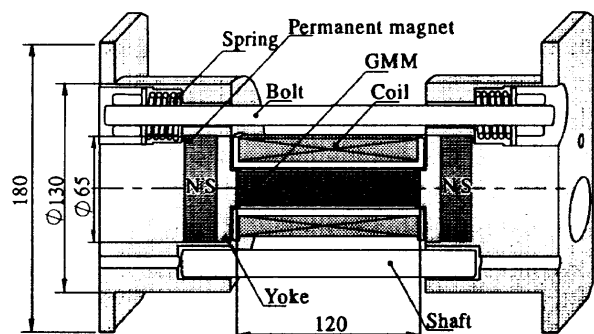
Fig. 4 Structure of the vibrator using giant magnetostrictive material (unit: mm).
