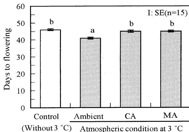
Fig. 4. The effect of atmospheric conditions at 3°C on the number of days to flowering of 'Aladdin' corms. Corms were packed with wet vermiculite in perforated polyethylene bags (0.04 mm thick) and placed under ambient or controlled atmosphere (CA) at 3% O 2 , 3% CO 2 and 94% N 2 at 3°C for 4 weeks. To make a modified atmosphere (MA), bags containing the corms were sealed and kept at 3°C. Corms were then planted in pots, exposed to 9°C for 6 weeks, and the plants were grown at 21°C. Means were separated by Tukey's HSD test ( P=0.05 ).
