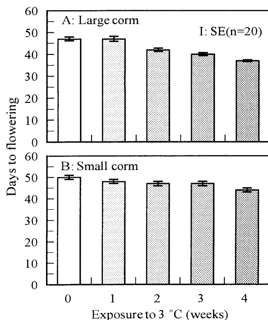
Fig. 1. The effect of the duration of the 3 °C treatment on large and small corms of 'Aladdin' on the number of days to flowering at 21 °C. Corms were planted, exposed to 3 °C for 0–4 weeks prior to 9 °C for 6 weeks, and then grown at 21 °C.
