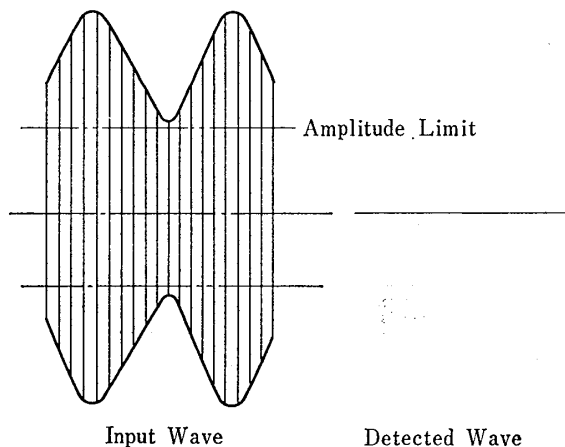
Fig. 6 Input Wave Over Amplitude Limit
