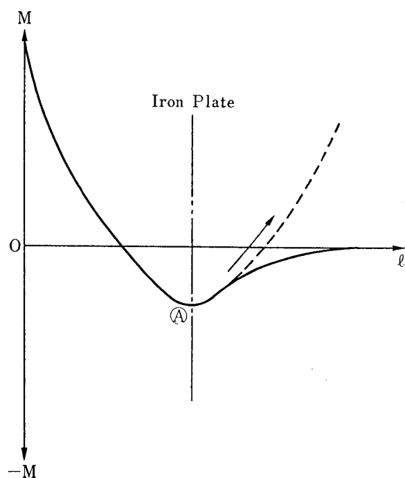
Fig. 3 Mutual Inductance
