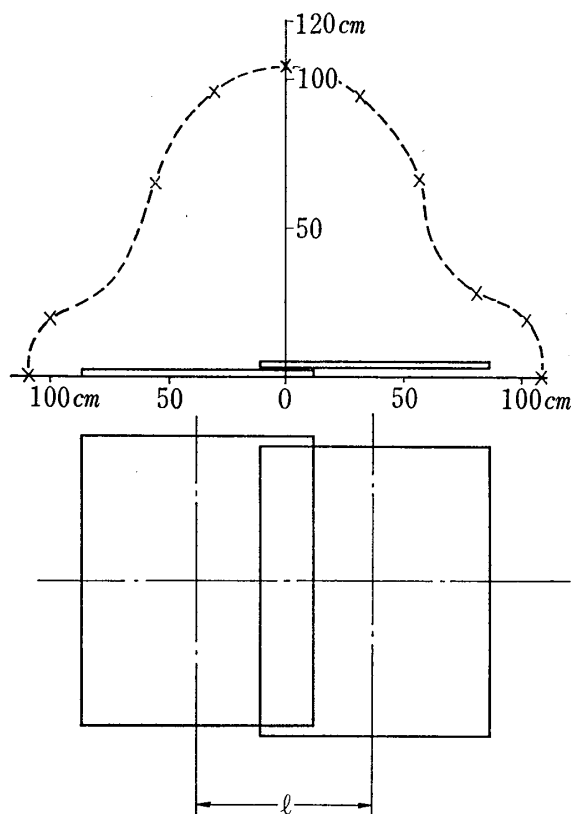
Fig. 4 Sensing Coil and Sensing Area
