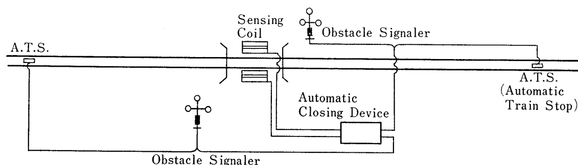
Fig. 7 Layout of Automatic Crossing System
