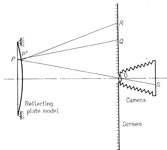
Fig. 4 Principle of Ligtenberg's method
