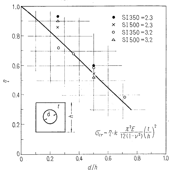
Fig. 14 Critical shearing stress versus opening ratio
