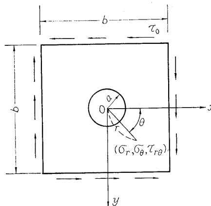
Fig. 2 Square plate with central circular hole
