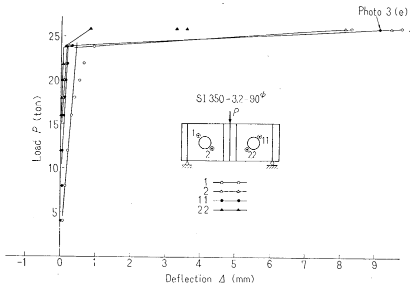
Fig. 12(b) Load-deflection curves
