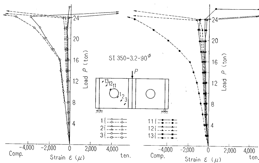
Fig. 10(a) Load-strain curves
