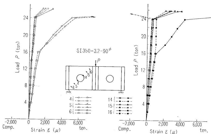
Fig. 10(b) Load-strain curves
