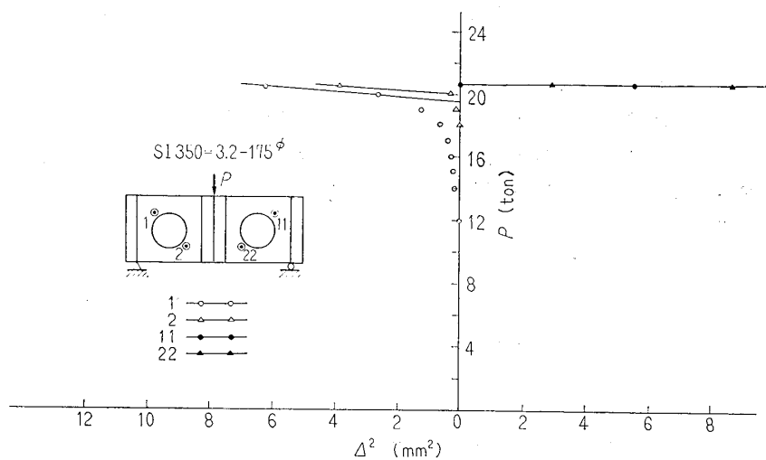
Fig. 13 P-\Delta^2 curves
