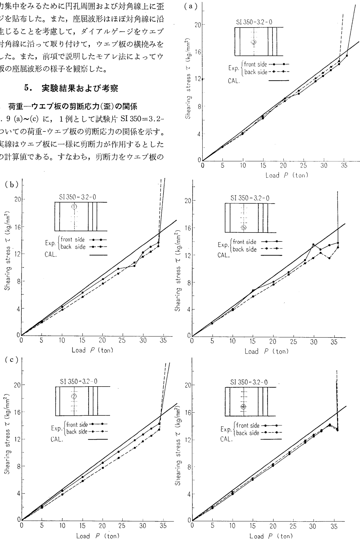
Fig. 9 Load versus shearing stress in web
