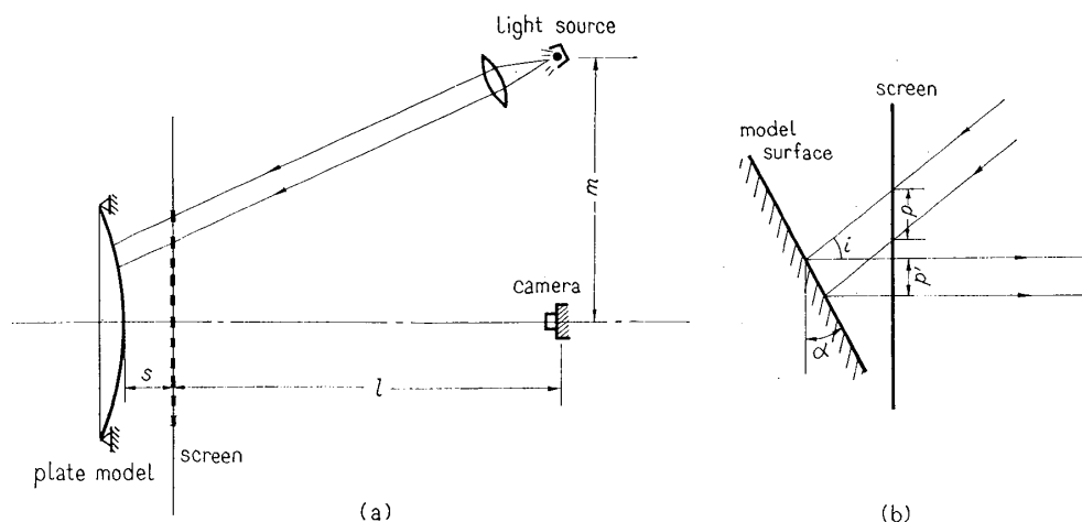
Fig. 5 Schematic representation of moiré method.
