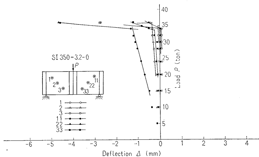
Fig. 12(a) Load-deflection curves
