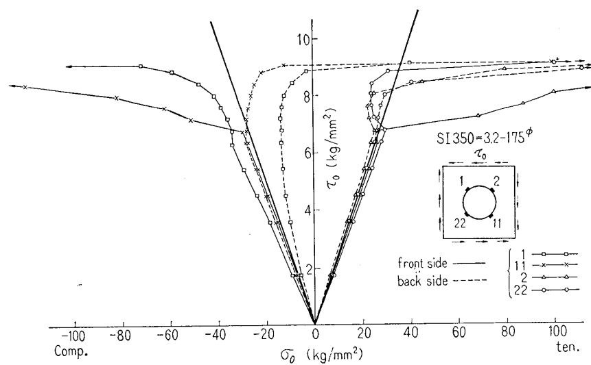
Fig. 11(b) Shearing stress versus tangential stress around hole
