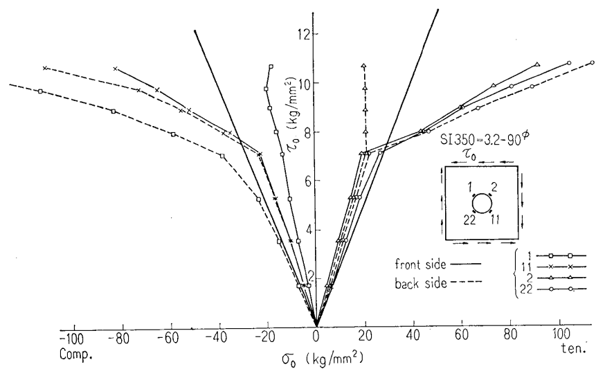
Fig. 11(a) Shearing stress versus tangential stress around hole
