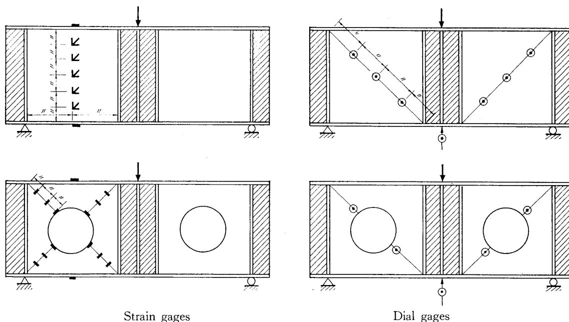
Fig. 8 Strain gage and dial gage locations on plate girders
