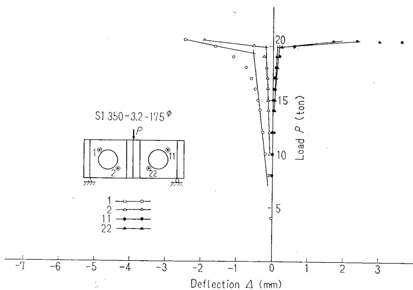
Fig. 12(c) Load-deflection curves
