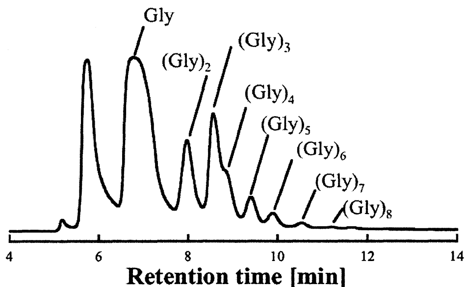
Fig. 2. Chromatogram of the products in the sample that reacted from 1 \text{ mol L}^{-1} glycine aqueous solution at 270^\circ\text{C} and 10 MPa.
