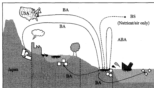
Fig. 2. Illustrational presentation of biostimulation (BS), bioaugmentation (BA), autochthonous bioaugmentation (ABA) treatments. In BS (broken arrow), only nutrients and/or oxygen are introduced to soils to enhance the activity of native contaminants-degrading microorganisms. Foreign microorganisms derived from the various places are added to contaminated sites in BA. In ABA, native (autochthonous) microorganisms are used and these organisms should be enriched under the conditions mimicking the sites, where ABA will be implemented. Open symbols with different shape indicate individual site-specific oil-degrading microorganisms and/or their mixture, whose routes of transfer are shown by the solid arrow. Native microorganisms for ABA are shown by the open circle in this figure. See Figure 3 for details of BA, BA and ABA.
