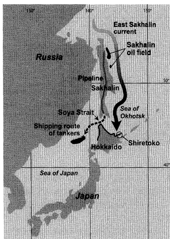
Fig. 4. The locations of Hokkaido and Sakhalin Islands. The Hokkaido coastlines that are at risk of oil contamination from the Sakhalin oil fields are shown by the solid line. This figure is from reference 31 and has been modified with permission.
