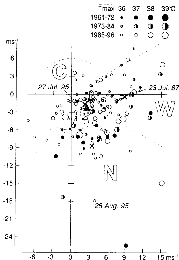
Fig. 6 Distribution of G on days with \overline{T_{\max}} \geq 36^\circ\text{C} , where G is geostrophic wind corresponding to surface pressure gradient and \overline{T_{\max}} is the highest value of T_{\max} among the eight JMA stations in the Kanto plain. Dotted lines show the boundaries between W-, N- and C-types. The average of G for each type is shown in "x".
