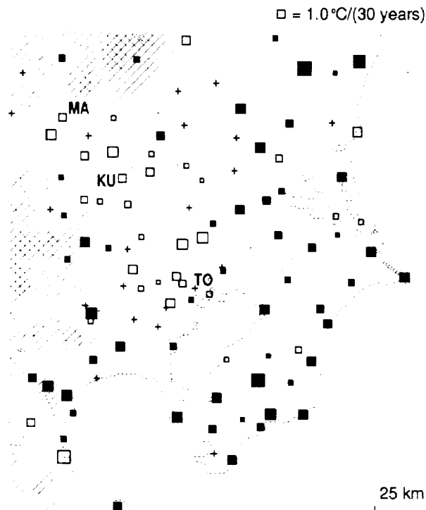
Fig. 4 Distribution of long-term change rates of A_{\max} during the period 1946-76. Open and closed squares indicate positive and negative trends, respectively, with their areas proportional to the absolute values of change rates. Crosses indicate change rates less than \pm 0.2^{\circ}\text{C}/(30\text{ years}) . Hatching indicates the area above 600 m and 1200 m m.s.l. with increasing tone.
