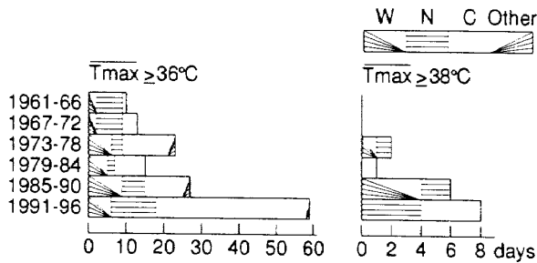
Fig. 9 Changes in the number of days with T_{max} \geq 36^\circ\text{C} and T_{max} \geq 38^\circ\text{C} stratified by prevailing wind types.
