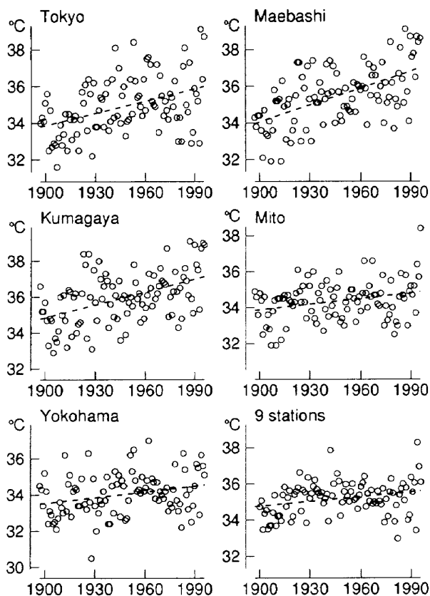
Fig. 3 Long-term changes in annual extreme maximum temperature ( A_{\max} ). The result for "9 stations" indicates the average for nine inland stations in central Honshu (Yamagata, Fukushima, Nagano, Takayama, Matsumoto, Gifu, Iida, Kofu and Hikone). Dashed lines indicate the linear regression obtained from the least-squares condition in Eq. (1).
