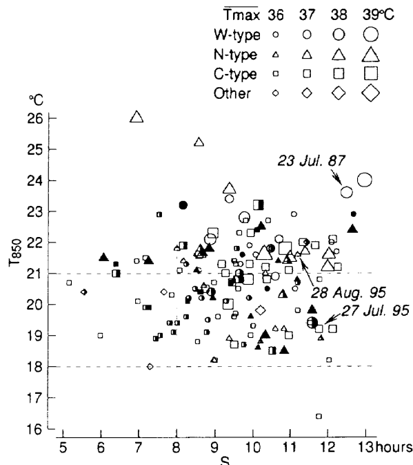
Fig. 7 Plot of the 850 hPa temperature ( T_{850} ) and duration of sunshine ( S ) on days with \overline{T_{\max}} \geq 36^\circ\text{C} . Open, half-filled and filled symbols correspond to 1961-72, 1973-84 and 1985-96, respectively.
