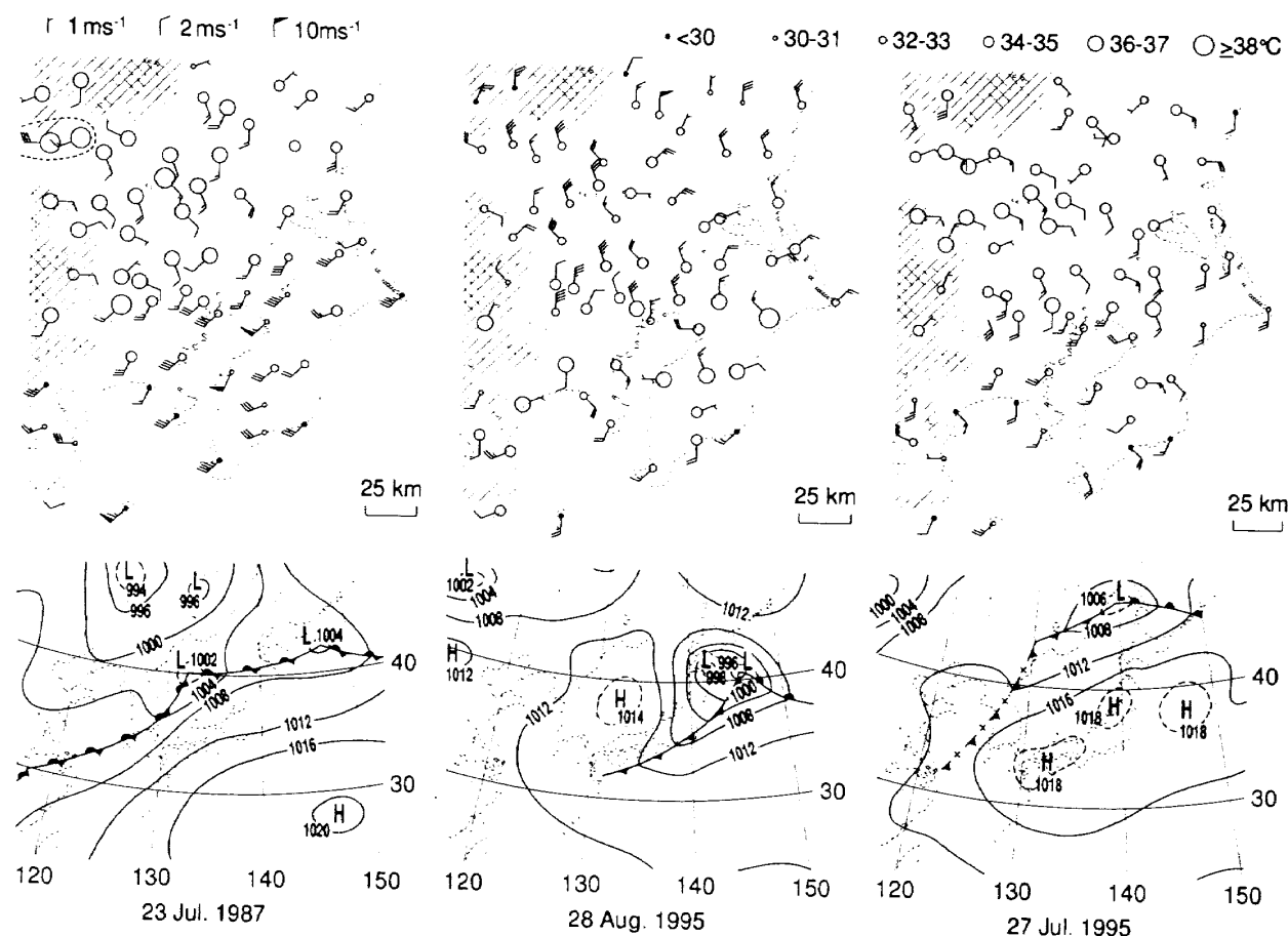
Fig. 5 Upper : Distribution of T_{\max} and surface wind at 15 JST on three selected days with extremely high temperature. The legend “30-31” indicates “ 30.0^{\circ}\text{C} \leq T_{\max} \leq 31.9^{\circ}\text{C} ”. Lower : Surface weather maps on these days.
