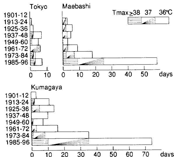
Fig. 2 Number of days with maximum temperature ( T_{\max} ) of 36°C or more in each twelve-year period. The legend "36" in the upper right corner means " 36.0^{\circ}\text{C} \leq T_{\max} \leq 36.9^{\circ}\text{C} ".
