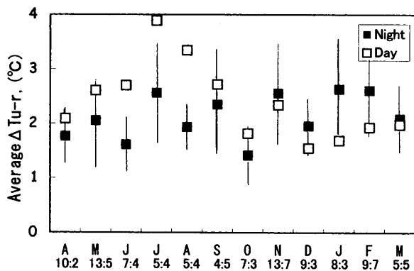
第6図 Seasonally change of monthly mean heat island intensity in Nozawa & Nakagomi settlement.
