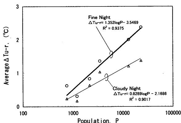
第4図 Relation between settlement population and the average of nighttime heat island intensity. ○: Fine day, △: Cloudy day.
