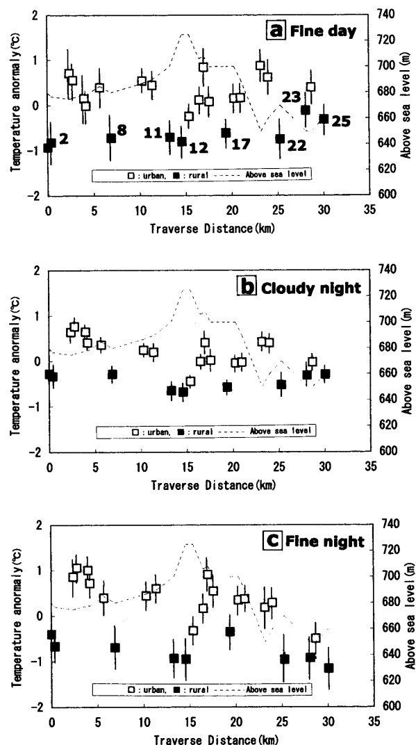
第3図 Traverse distance from station No.1 and nocturnal mean temperature in observation stations. □ : Urban (settlement), ■ : Rural.
