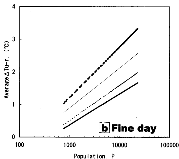
第7図 Relation between settlement population and the average of heat island intensity in seasonally classification.
