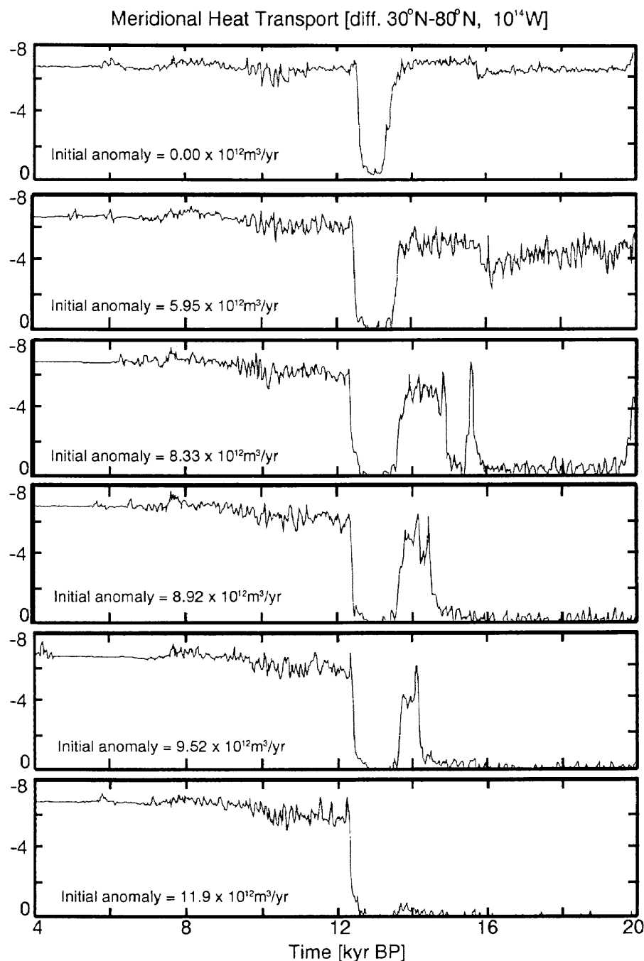
Fig. 5. Results from experiment I. The individual plates present the difference of the meridional heat transport between 30°N and 80°N in the Atlantic Basin for the values of the initial background anomaly depicted on Fig. 3 (since the transport is taken as positive for southward direction, northward heat transport corresponds to the negative sign). The amplitude of this heat transport is proxy for the intensity of NADW.
