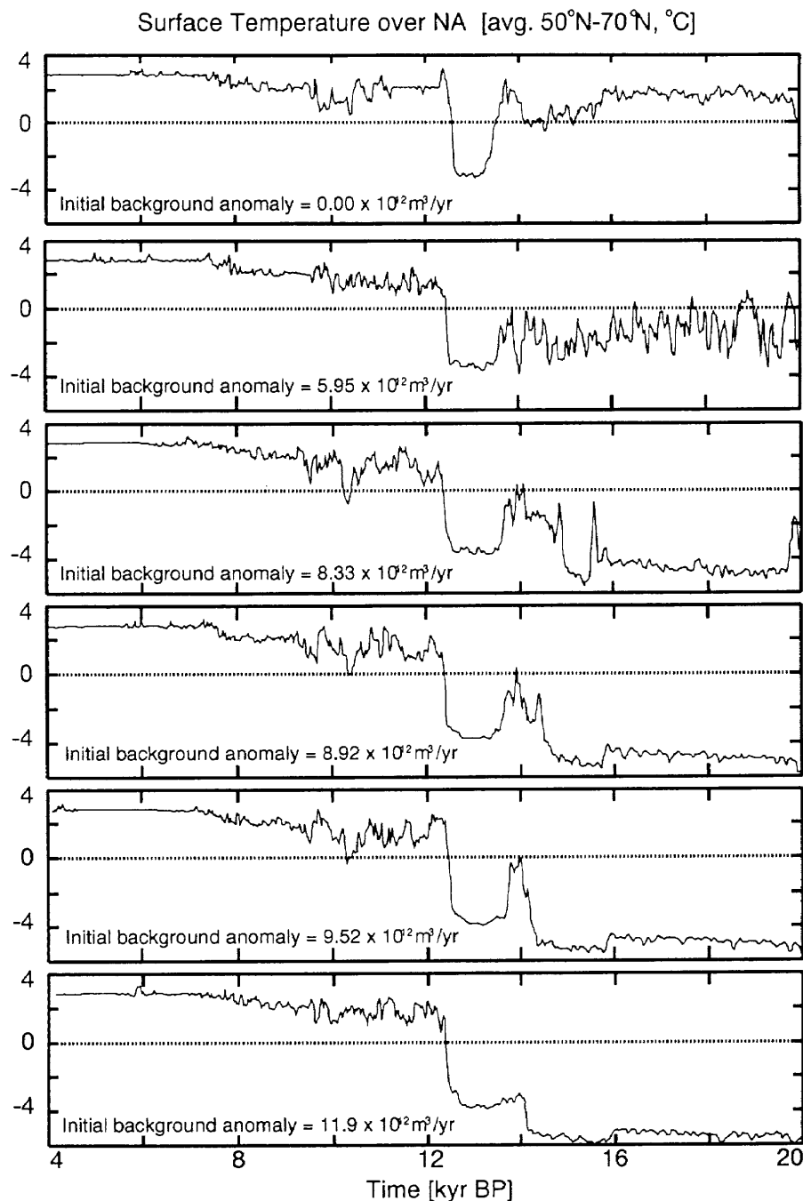
Fig. 7. Results from experiment I. The individual plates present time series of sea surface air temperature averaged between 50°N and 70°N over the Atlantic for the same sequence of initial background components of the freshwater forcing anomaly for which results are shown on Fig. 5.
