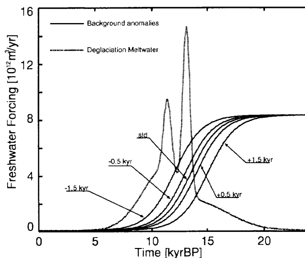
Fig. 4. Model deglaciation histories in terms of meltwater flux in the interval between 0 and 24 kyr BP for the second set of deglaciation experiments. In this set of experiments the sea level related contribution to the meltwater flux is held constant but the timing of reduction of the background anomaly is varied.
