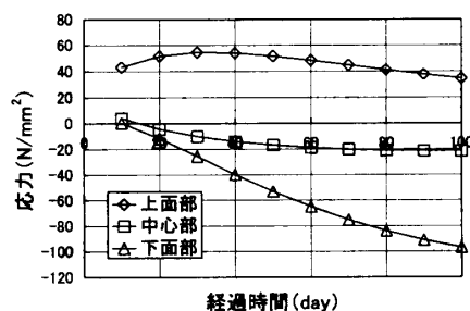
図-6 応力履歴 (R.H.50-10)
