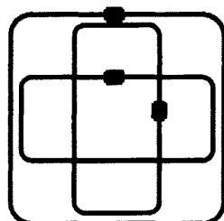
図-2 溶接閉鎖型筋
