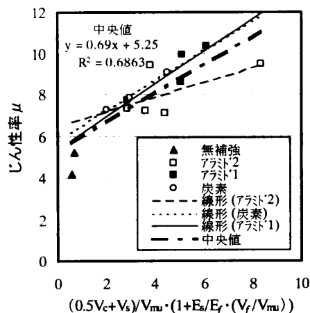
図-9 (0.5V_c+V_s)/V_{mu} \cdot (1+E_s/E_f \cdot (V_f/V_{mu})) とじん性率の関係
