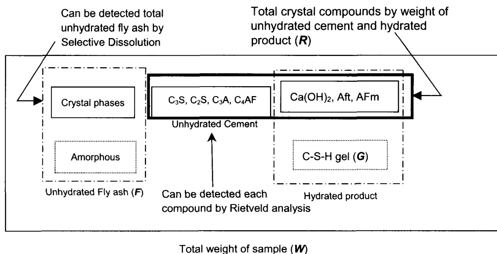
Fig 1. Superposition of Rietveld analysis and selective dissolution
