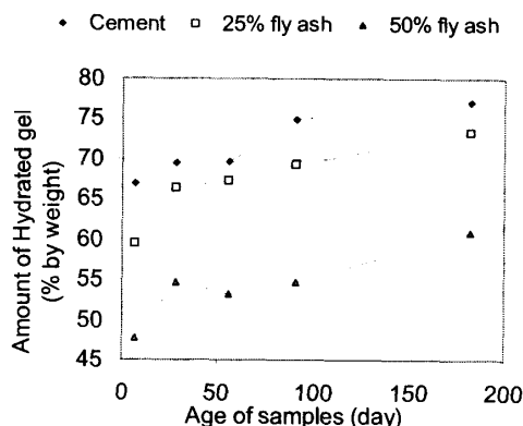
Fig. 7 The amount of hydrated gel at different age
