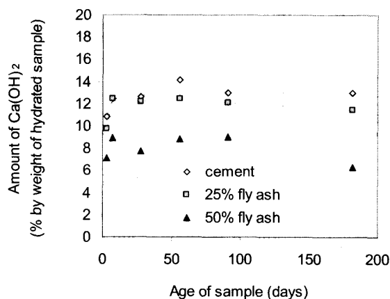
Fig. 5 The amount of \text{Ca(OH)}_2 at different age
