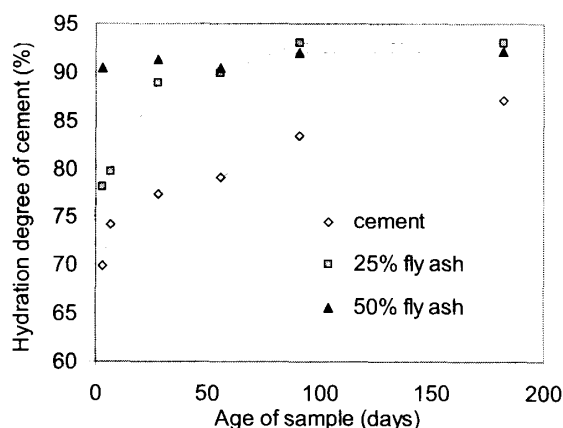
Fig. 4 Hydration degree of cement
