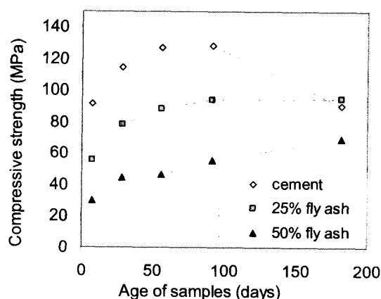
Fig. 8 Compressive strength as a function of time
