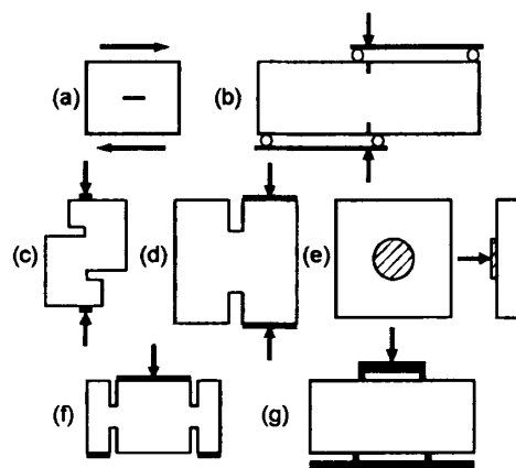
Figure1 Different test configurations
