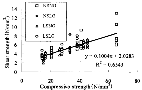
Figure 3 Shear strength and compressive strength relation
