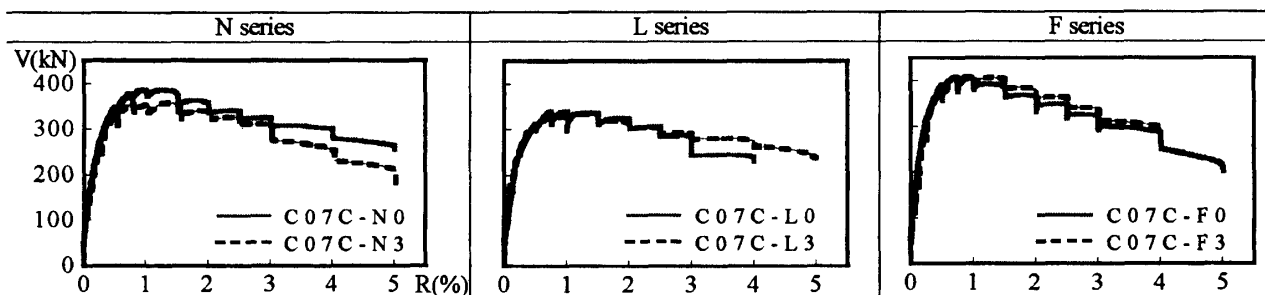
Fig. 9 Comparison of measured skeleton curves.
