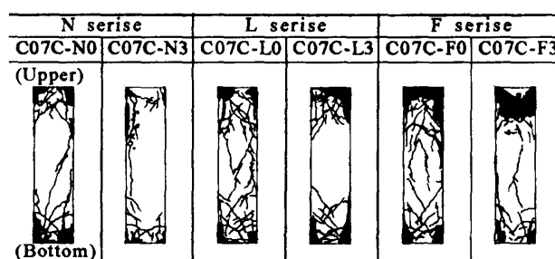
Fig. 8 Observed final cracking patterns of seaside face.
