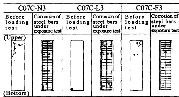
Fig. 3 Cracks of cover concrete and corrosion of steel bars in RC column specimen.
