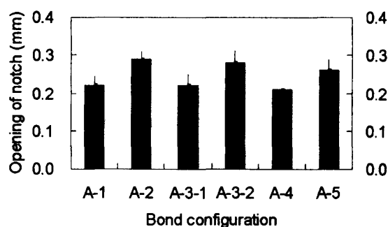
Fig. 11 Crack performance at P = 10 kN
