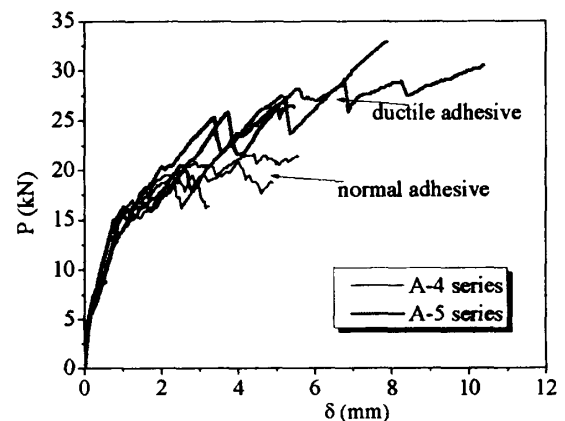
Fig.7 P-\delta curves of CFSS strengthened beams with unique adhesive bonding
