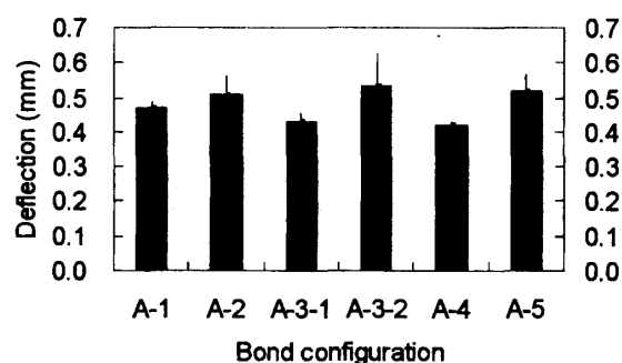
Fig. 10 Member deflection at P = 10 kN
