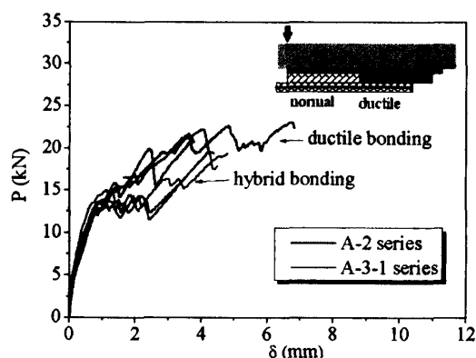
Fig.8 P \sim \delta curves of strengthened beams with the hybrid use of two adhesives
