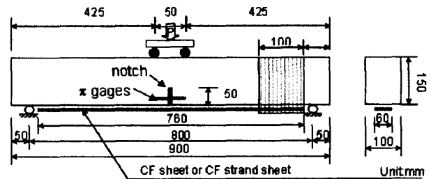
Fig.3 Geometry of specimens
