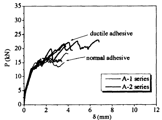
Fig.6 P-\delta curves of CCFS strengthened beams with unique adhesive bonding
