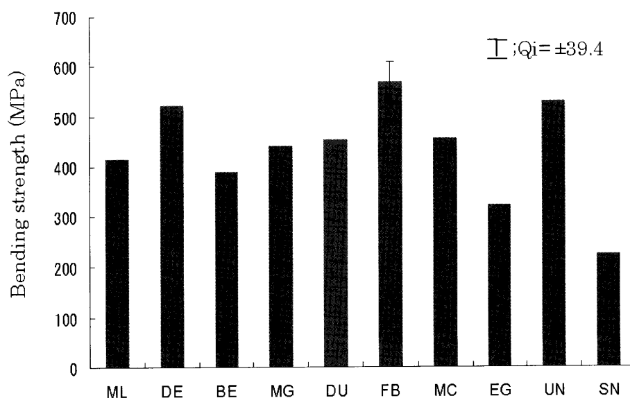
Fig. 1 Effects of bonding agents on bending strength.
