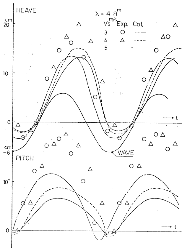
Fig. 12 Result of simulation and model test (2)
