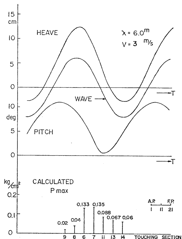
Fig. 21 Simulated ship motion (does not jump)
