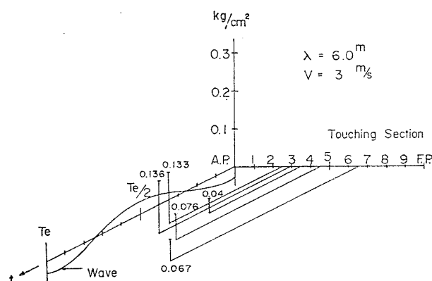
Fig. 24 Calculated impact pressure (does not jump)
