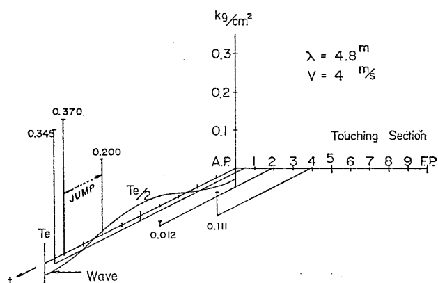
Fig. 22 Calculated impact pressure (jump)
