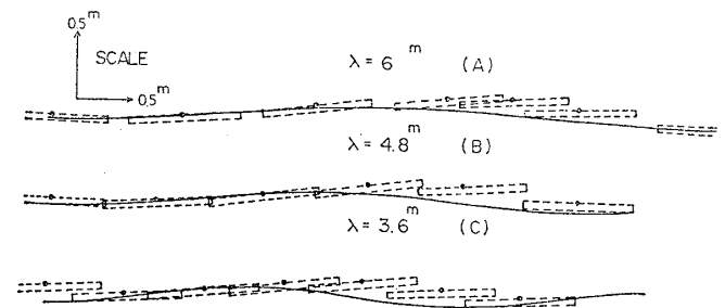
Fig. 14 Simulated ship motion in the head sea ( V_s=5\text{m/s} )
