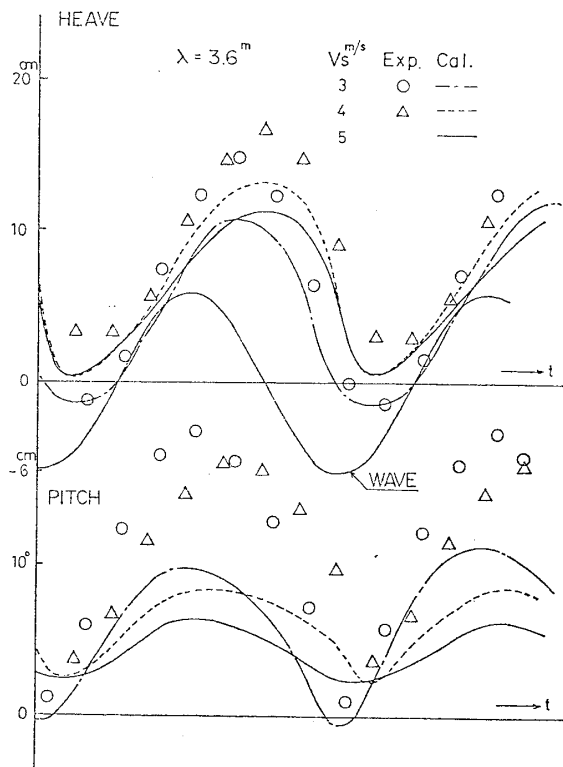
Fig. 11 Result of simulation and model test (1)
