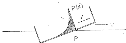
Fig. 4 Longitudinal pressure distribution
