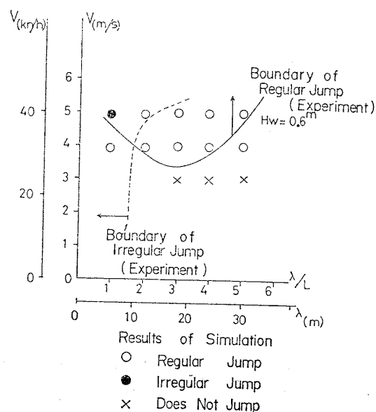
Fig. 9 Criteria of jumping
