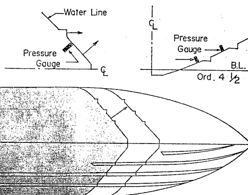
Fig. 26 Pressure transmission along with sinkage
