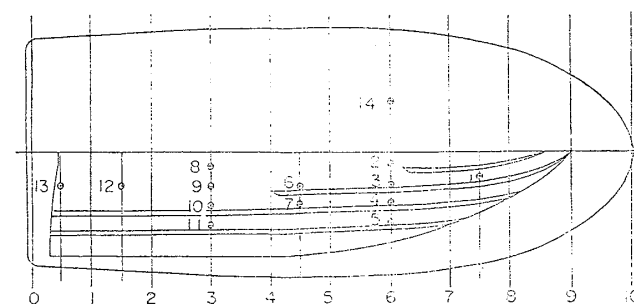
Fig. 7 Position of pressure gauges
