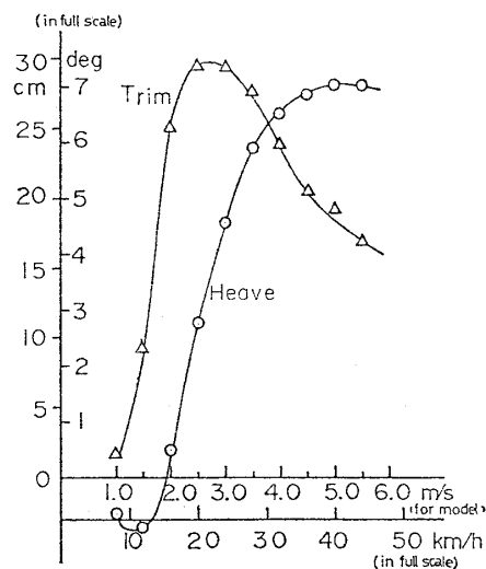
Fig. 5 Running trim and heave
