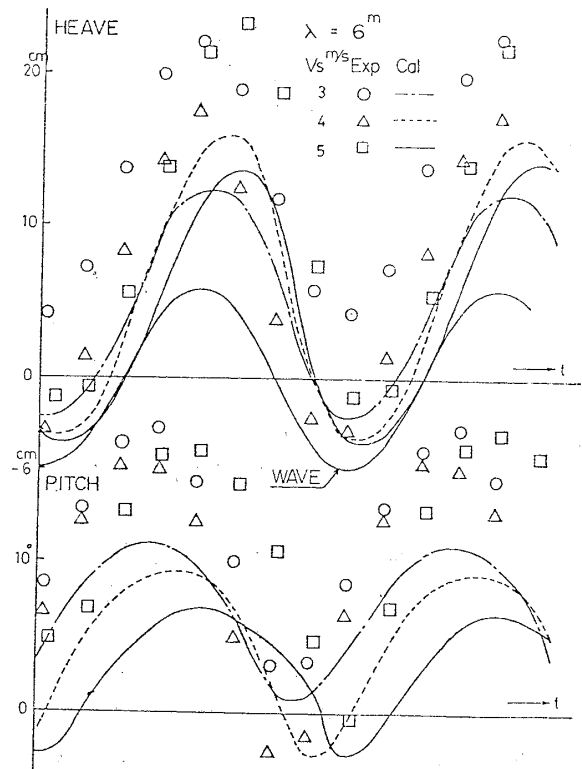
Fig. 13 Result of simulation and model test (3)
