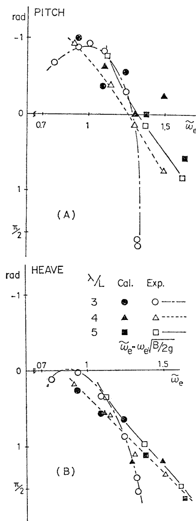
Fig. 16 Phase lags of heave and pitch
