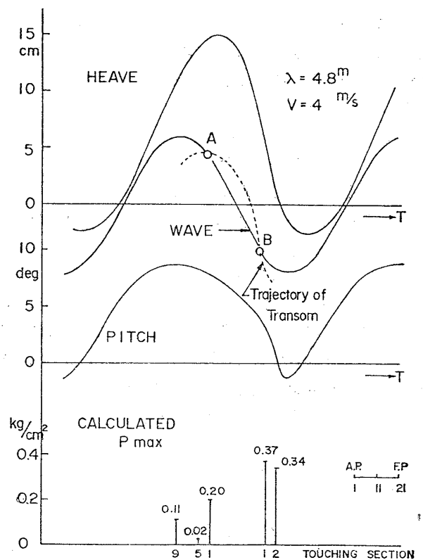
Fig. 19 Simulated jumping phenomena and calculated impact pressure
