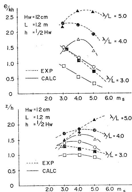
Fig. 15 Pitch and heave responses in waves
