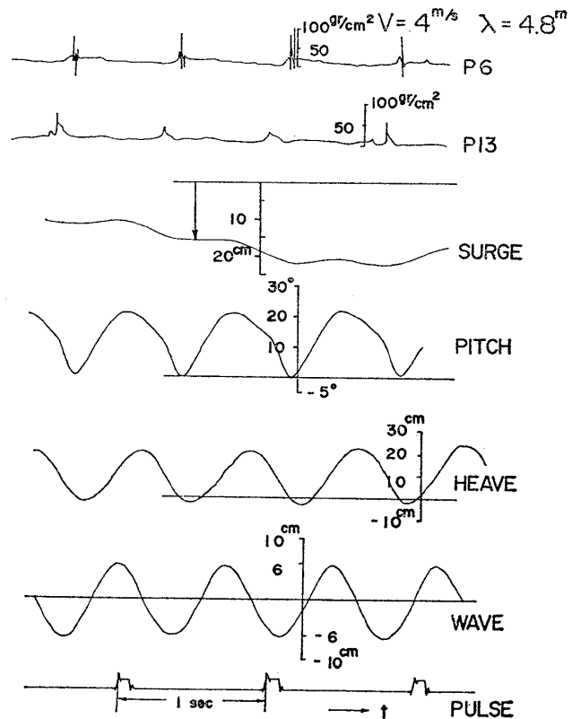
Fig. 18 Record of model test showing jumping phenomena
