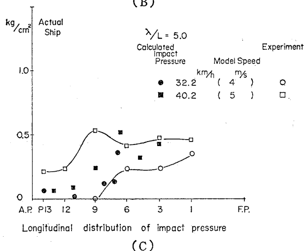
Fig. 17 Longitudinal distribution of a impact pressure
