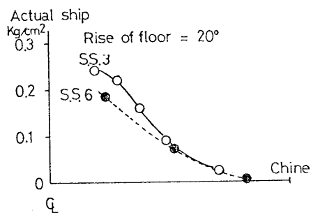
Fig. 28 Calculated impact pressure lateral distribution ( \lambda=6.0\text{m} , V_s=5\text{m/s} )
