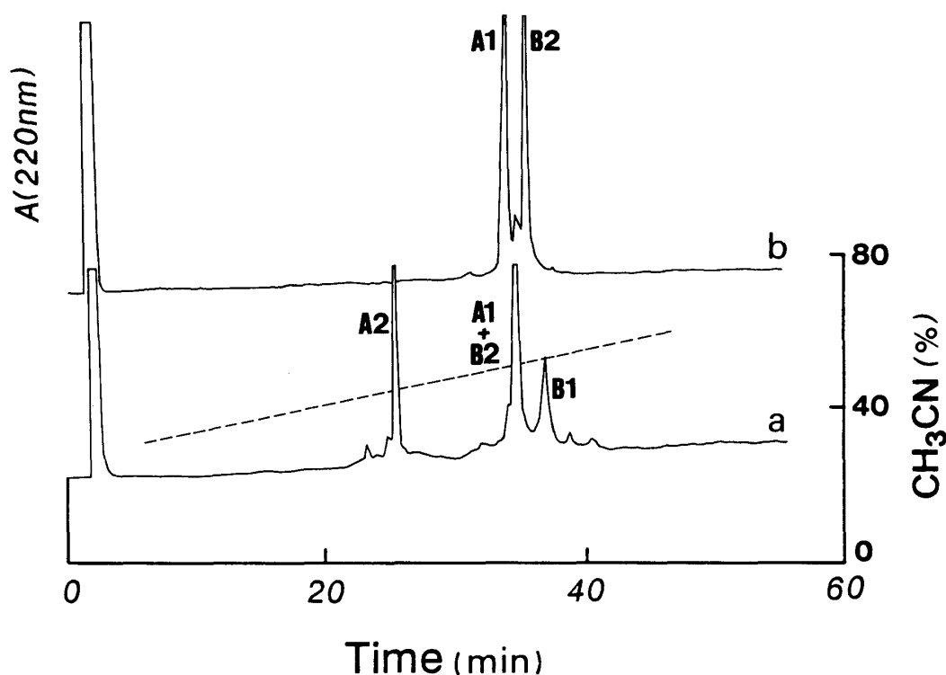
FIG. 2. Separation of the constituent chains of the 440 kDa hemoglobin from Slender vestimentifera gen. sp.1 by reverse-phase chromatography. The column (Cosmosil 5C 18 -300) was eluted with a linear gradient of acetonitrile in 0.1% TFA at a flow rate of 1 ml/min. (a), reduced 440 kDa hemoglobin; (b), rechromatography of chains A1 and B2 after carboxymethylation.
