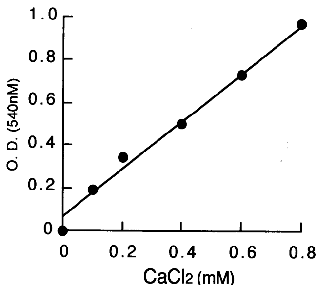
Fig. 2. Optical density of Ca-precipitate by pyroantimonate. This shows pyroantimonate can detect calcium down to 0.1 mM. Optical density (OD) was measured through a 540 nm wavelength filter.
