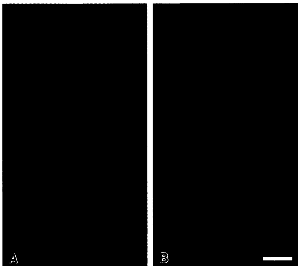
Fig. 2. FISH with Paramecium genomic DNA probe for C5 antigen or a cosmid probe from human in Paramecium nuclei. Cells were denatured at 85°C for 10 min in accordance with the conventional. FISH signals (green) and its corresponding DAPI staining image (blue) were merged. A: FISH with 1.3 kb parametecium genomic DNA probe for C5 antigen. B: FISH with 40 kb cosmid probe of human chromosome 22q11.2. Sections were captured at 5 \mu m depth from the nuclear surface. All images were deconvoluted to remove the unfocused haze. Bar, 10 \mu m.
