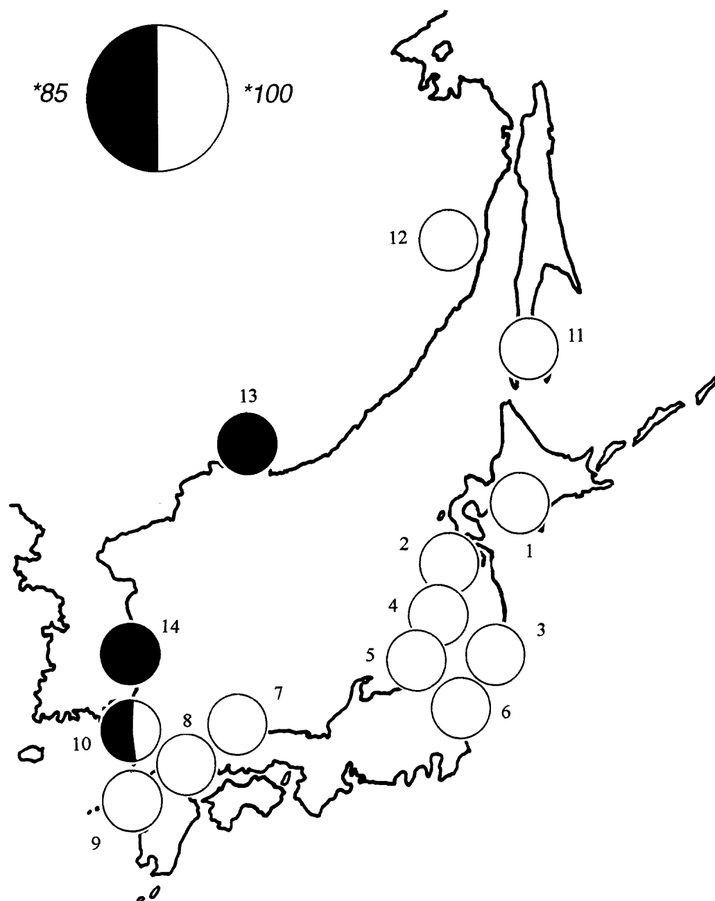
Fig. 3. Distribution of Prot-2* alleles (*100, *85) in Tribolodon hakonensis . Population numbers are shown in Table 1.
