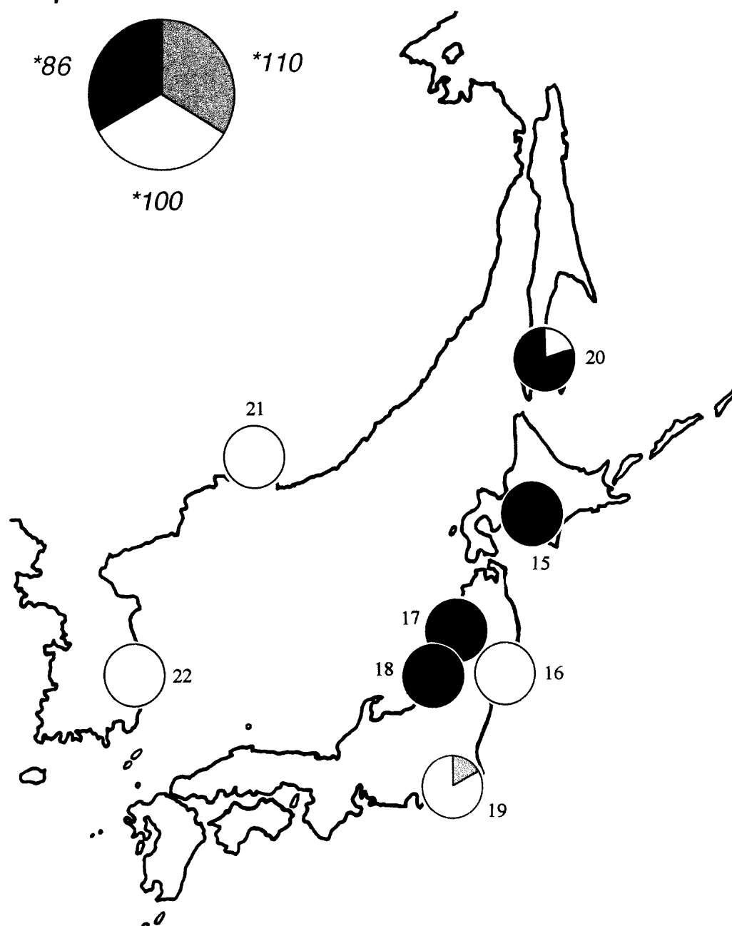
Fig. 4. Distribution of Gpi-1* alleles (*110, *100, *86) in Tribolodon brandtii . Population numbers are shown in Table 1.
