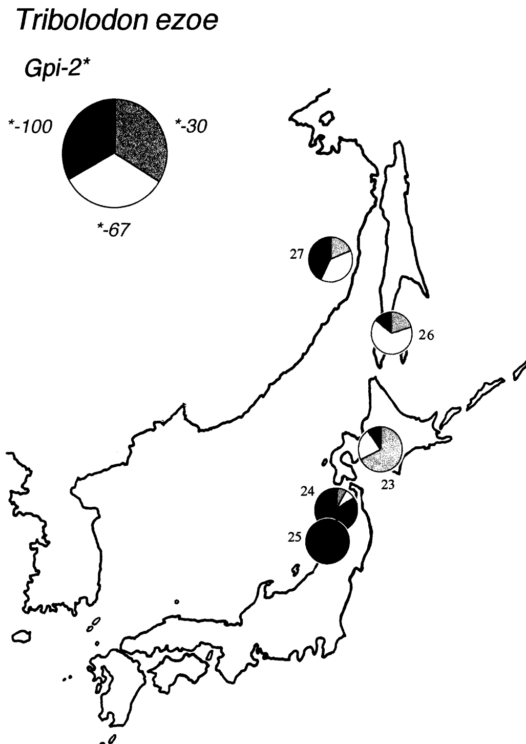
Fig. 5. Distribution of Gpi-2* alleles (*-30, *-67, *-100) in Tribolodon ezoe . Population numbers are shown in Table 1.
