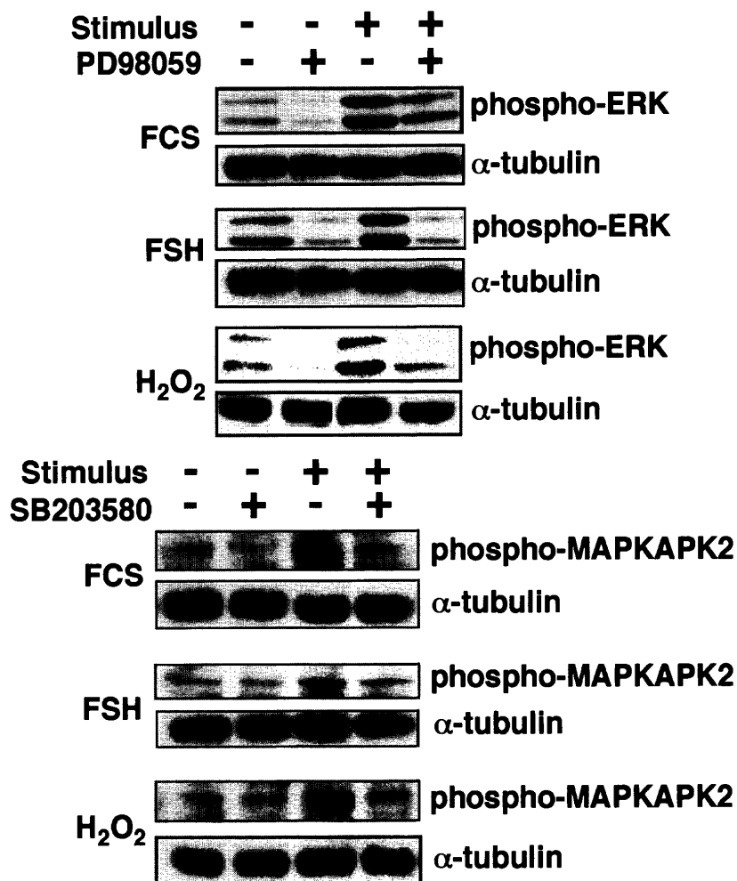
Fig. 2. Effectiveness of PD98059 and SB203580. Cells cultured in medium containing 0.3% serum for 6 hr were stimulated with 200 ng/ml FSH, 10% serum, or 100 \mu M H_2O_2 in the presence and absence of 50 \mu M PD98059 or 20 \mu M SB203580 for 5 min. The inhibitors were added to the medium 30 min prior to the stimulation. Thereafter, the ERK1/2 and MAPKAPK2 activities were assessed by Western blotting using phospho-specific ERK1/2 and phospho-specific MAPKAPK2 antibodies. The same membrane was stripped and reprobed with an anti- \alpha -tubulin antibody. Data represent two separate experiments that yielded similar results.
