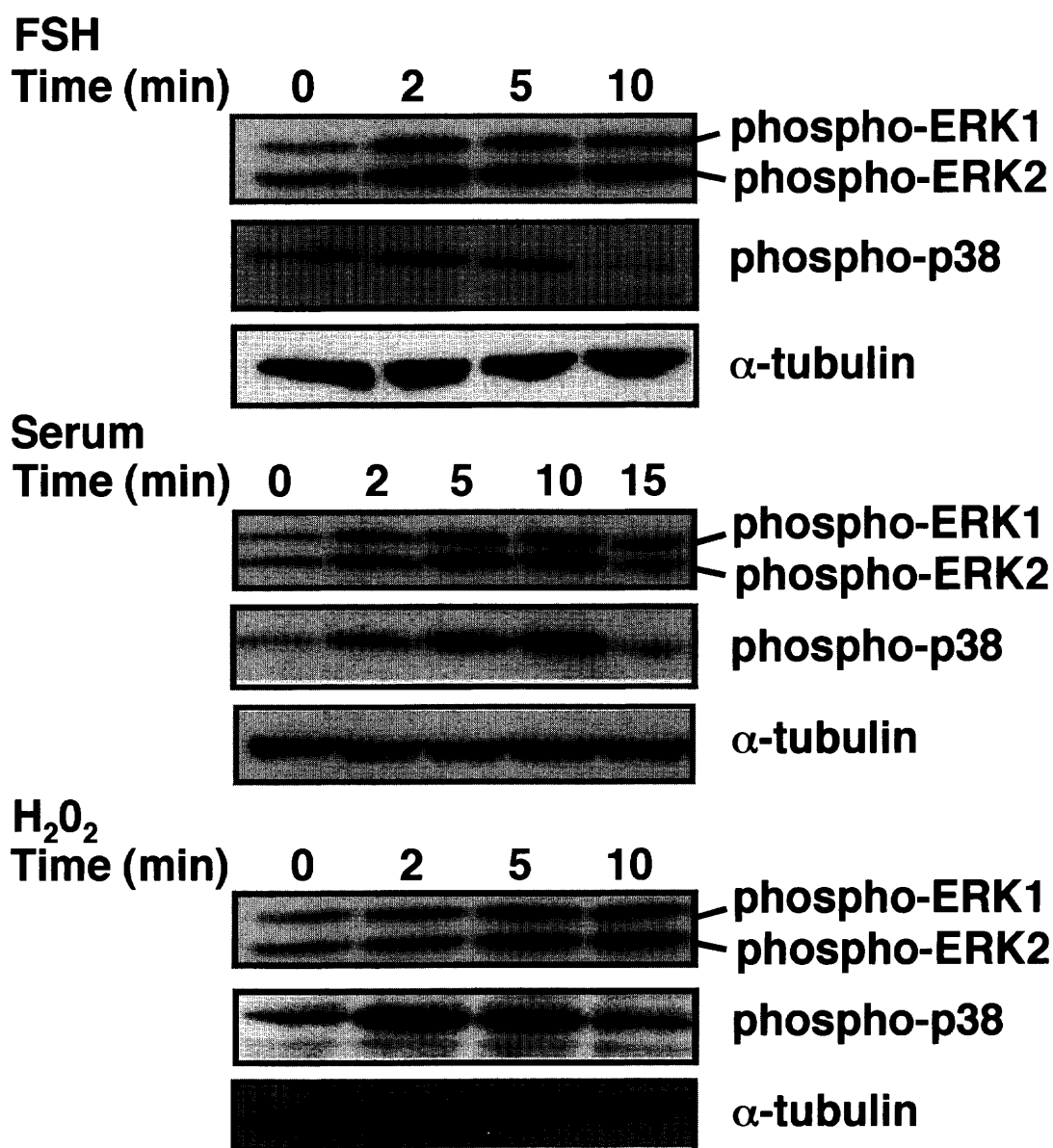
Fig. 1. Activation of ERK1/2 and p38 in response to FSH, serum, and H 2 O 2 . Cells cultured in medium containing 0.3% serum for 6 hr were stimulated with 200 ng/ml FSH, 10% serum, or 100 \mu M H 2 O 2 for the indicated periods. Thereafter, cell lysates (40 \mu g of protein) were loaded on 10% SDS-PAGE and immunoblotted using phospho-specific anti-ERK1/2, phospho-specific anti-p38, and anti- \alpha -tubulin antibodies as described in "Materials and Methods". The bands of \alpha -tubulin are indicated as internal control. The same membrane was reprobed in each panel. Data represent three separate experiments. Similar results were obtained in two other experiments.
