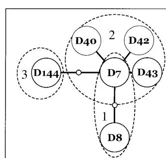
Fig. 3. Statistical parsimony tree of the haplotypes from D. nanus and D. moiwanus . Haplotypes are indicated by large open circles with haplotype codes (see Table 1 and Fig. 2). Mutational steps are represented by thick lines with small open circles representing intermediate haplotypes that did not appear in the samples. Haplotypes from the same locality are encircled by a dashed line, with the locality number indicated (see Table 1).
