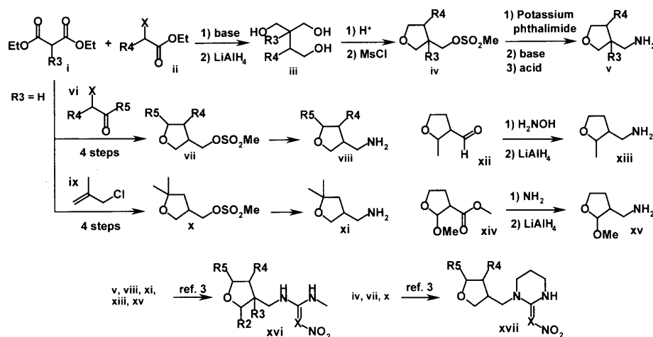
Fig. 3. Synthesis of substituted tetrahydro-3-furylmethyl derivatives xvi and xvii .
