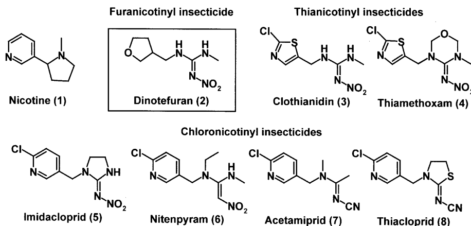
Fig. 1. Nicotine and Neonicotinoids.
