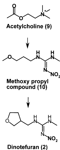
Fig. 2. Discovery of dinotefuran (2).
