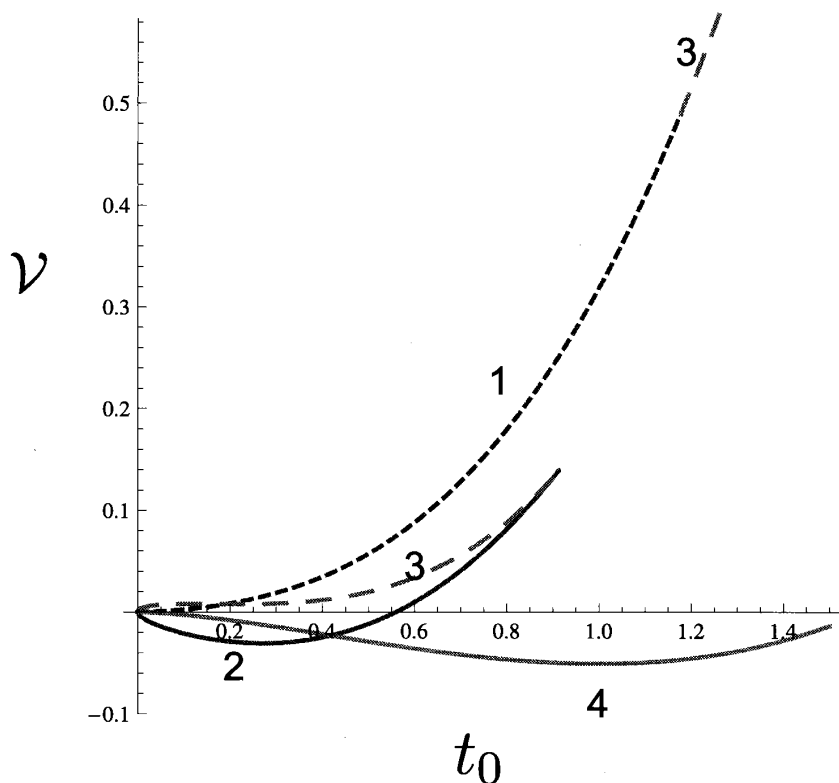
Fig. 1. Four branches of the effective potential \nu . We find local minimum in branches 2 and 4. Branch 3 consists of two disconnected curves.
