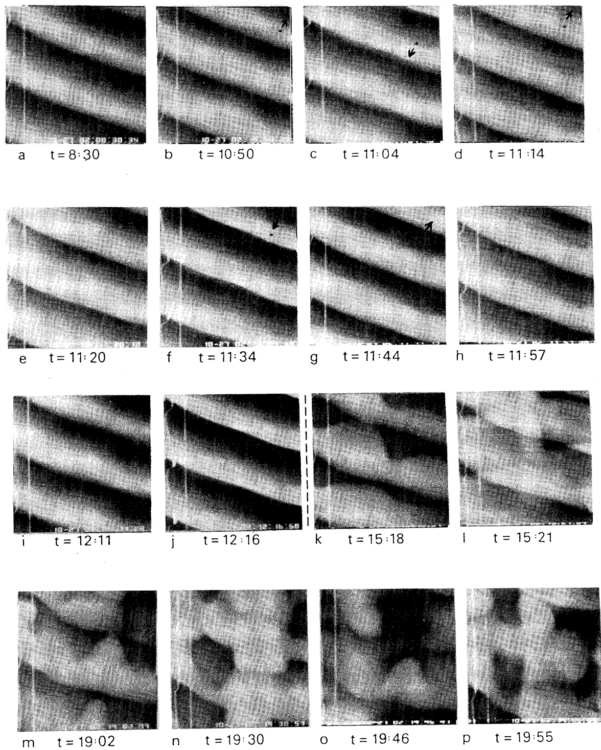
Fig.7 Image sequence of the temporal development of waves at 490nm under uncovered condition (without illuminated polystyrene particles).
