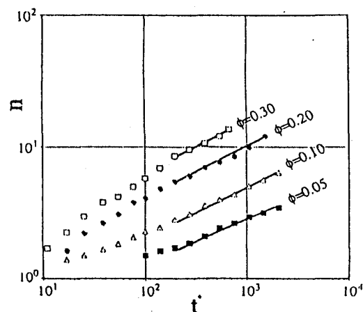
Fig.5. Graph showing the relationship between n , t^* and \phi , obtained from 2 dimensional ERF simulations.
