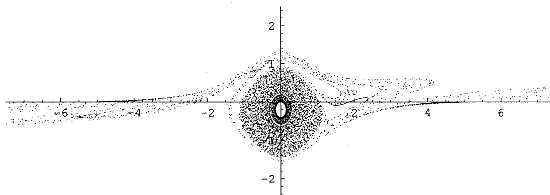
図4. Poincare断面 ( \omega = 0.45 , \alpha = 0.4 )
