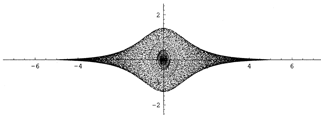
図3. Poincare断面 ( \alpha = 0 )
