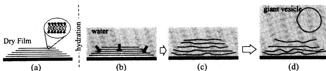
Figure 2: Hydration process of stacked bilayers. When the dry film (a) is hydrated, water molecules penetrate into the stack (b). Next, the multi-lamellar structure is swollen and reaches a quasi-stable state (c). Following, each bilayer gradually peels off from the stack to form a giant vesicle (d).
