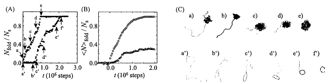
Figure 1: Time evolution of the number of collapsed monomers in the semiflexible block of a rod-coil copolymer (○) and a semiflexible homopolymer (△). Each polymer has N = 256 monomers, and a bending elasticity \kappa_s = 15 for the semiflexible parts. We change the attractive interaction at t = 0 to \epsilon = 0.8 . N_{\text{fold}} shows the number of monomers in the folded state. The bare data are shown in (A), while the mean evolution over 30 runs is shown in (B). Snapshots of the polymer conformation during the transition for a rod-coil copolymer (a-f) and a semiflexible homopolymer (a'-f') are shown in (C).
