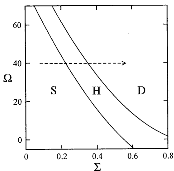
Figure 2: Mean-field phase diagram in the (\Sigma, \Omega) plane. \Sigma represents the reduced surface tension and \Omega the temperature-composition coupling parameter. The effect of increasing the surface tension is represented by the dashed right-hand arrow.
