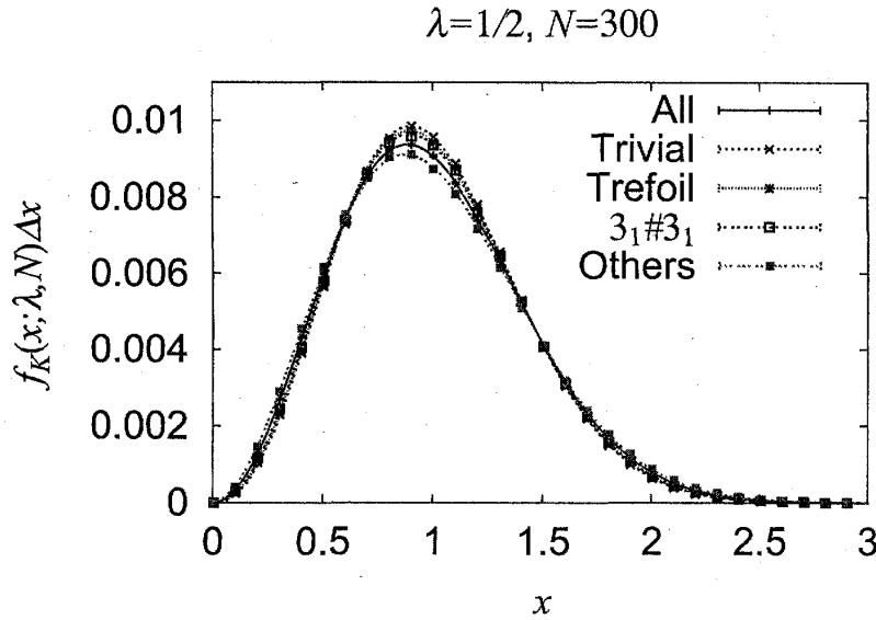
Figure 1: The probability distribution \tilde{f}_K(x; \lambda, N) for \lambda = 1/2 and N = 300 [13, 14]. For topological conditions, 0, 3_1 , 3_1 \# 3_1 , others and all , the \chi^2 per datum are given by 3.19, 1.30, 0.31, 2.85 and 0.17, respectively; the estimates of \theta_K are given by 0.300 \pm 0.004 , 0.225 \pm 0.003 , 0.169 \pm 0.003 , -0.164 \pm 0.003 and 0.0007 \pm 0.0005 , respectively.
