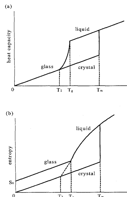
Fig. 1 (a) heat capacity vs temperature (b) entropy vs temperature
