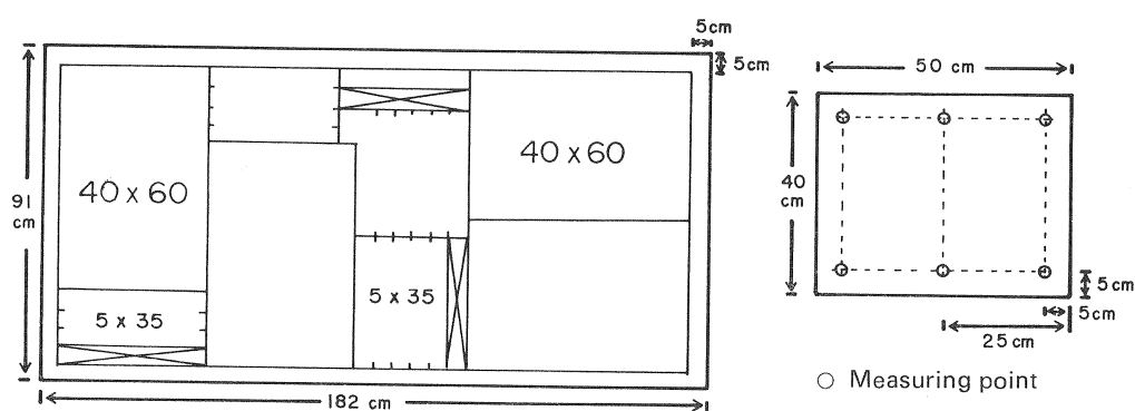
Fig. 2 試験片の採取方法および厚さの測定点 Cutting of specimens and measuring points for thickness.
