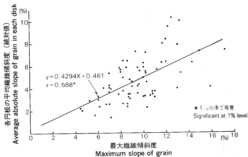
Fig. 4. 最大繊維傾斜度と平均繊維傾斜度 (絶対値) との関係 Relation between maximum slope of grain and average absolute slope of grain in each disk of sample trees.
