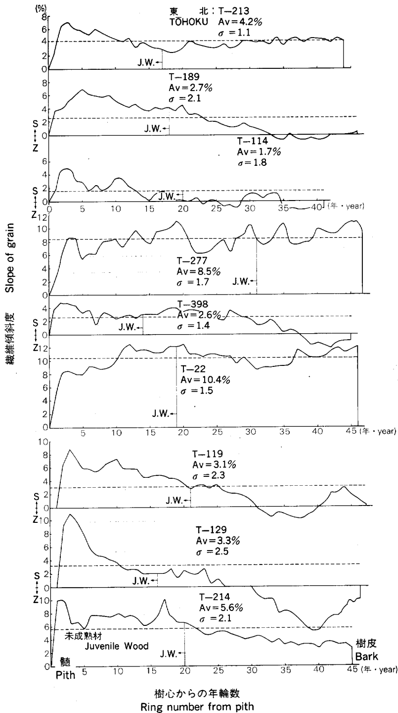
Fig. 1. 繊維傾斜度の樹心から外周までの各年の変化 (東北) Variation in the slope of grain of annual rings from pith to bark.
