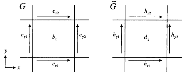
Fig. 3: Electric voltage drop - magnetic flux, and magnetic voltage drop - electric flux.
